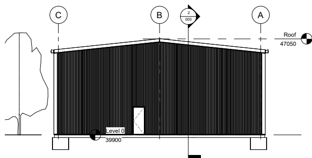
③ South 1 : 100
