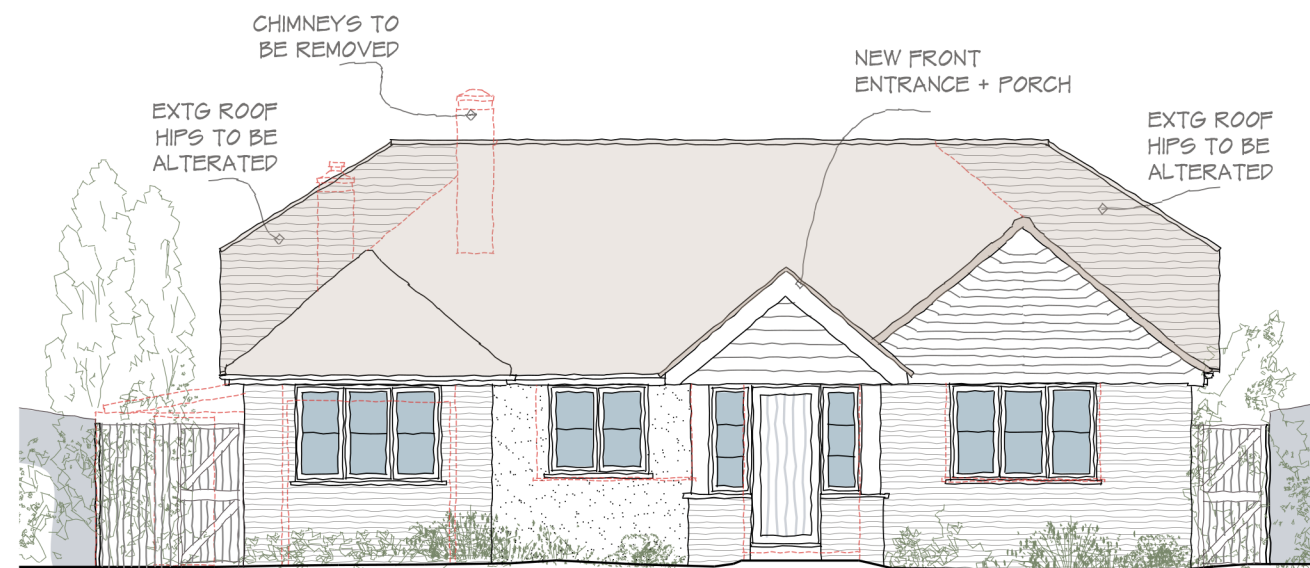
FRONT ELEVATION NORTH WEST - 1:100
