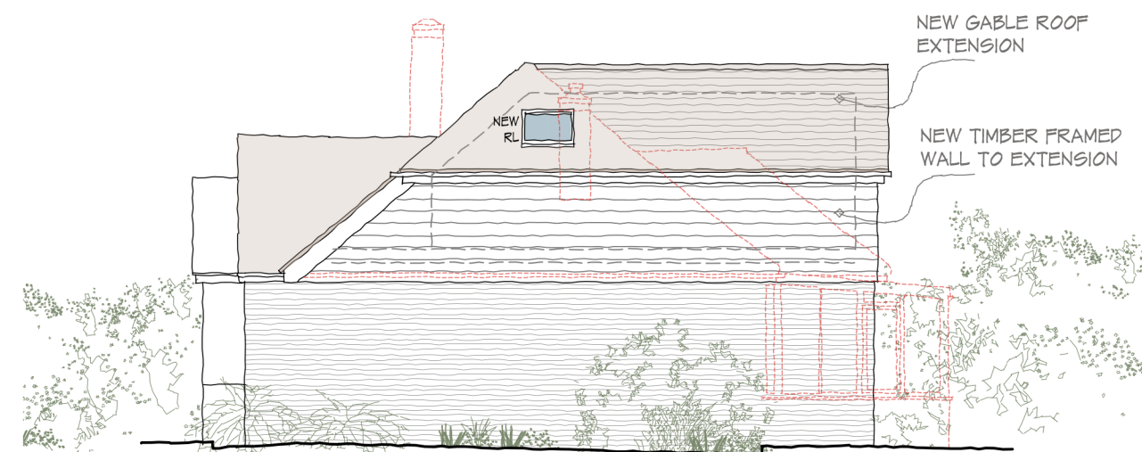
SIDE ELEVATION SOUTH WEST - 1:100
