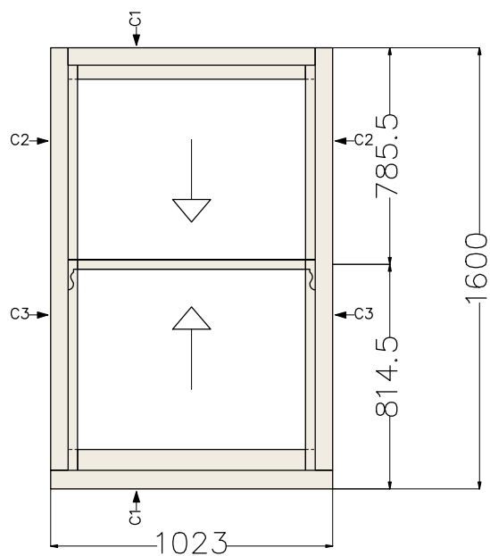
View from outside (scale 1:25)
