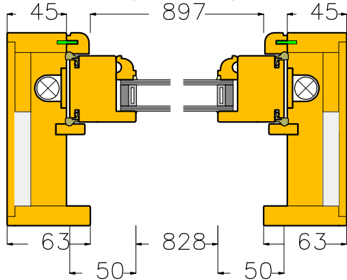
Section C3 (scale 1:4)
