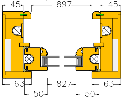
Section C2 (scale 1:4)
