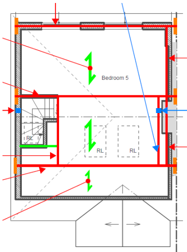
LOFT FLOOR PLAN
