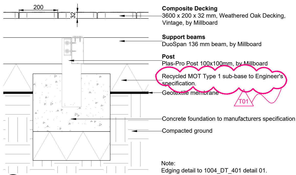
S4 Composite decking Scale: 1:10. Land. Spec.: Q55.380
