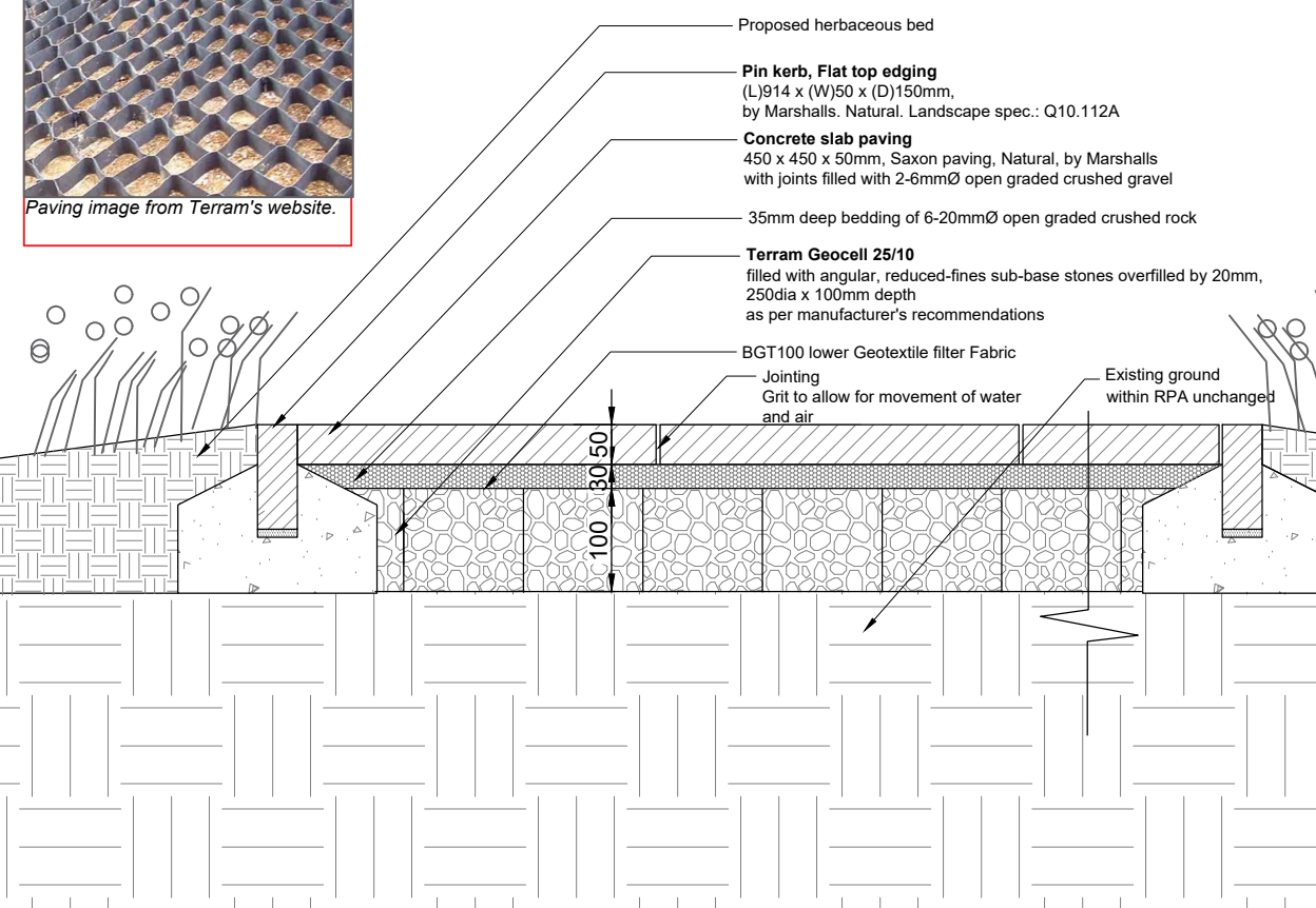
S12a No dig construction - concrete slab Scale: 1:10
