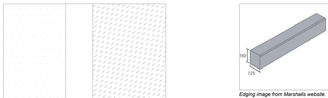
S11 Tactile blister paving Scale: 1:10. Land. Spec.: Q25.320
