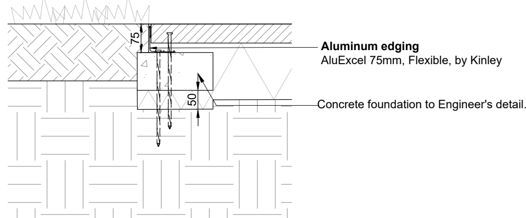
E2 Aluminum edging Scale: 1:10. Land. Spec.: Q30.560
