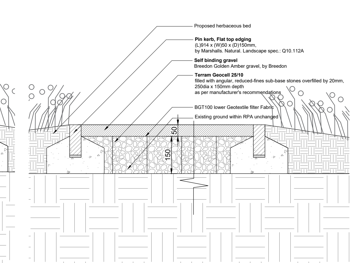
S12b No dig construction - self binding gravel Scale: 1:10
