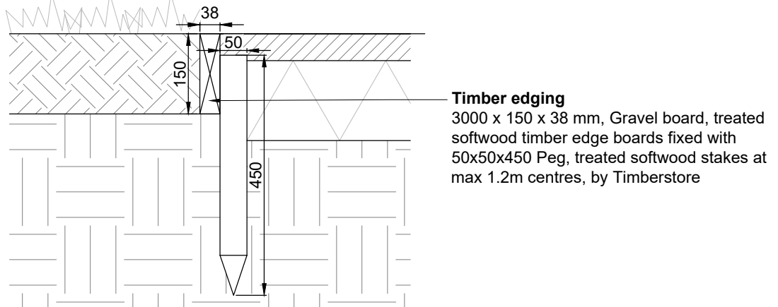
E1 Timber edging Scale: 1:10. Land. Spec.: Q23.310
