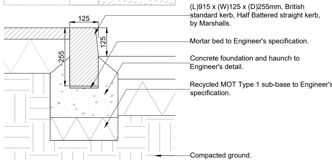
E7 Straight kerb Scale: 1:10. Land. Spec.: Q10.113
