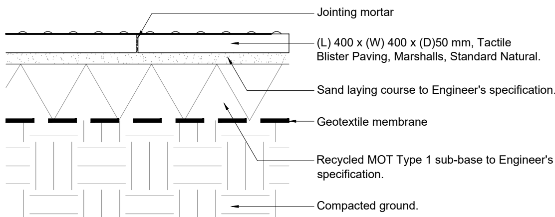
S11 Tactile blister paving Scale: 1:10. Land. Spec.: Q25.320
