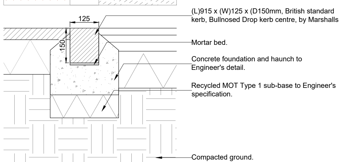
E5 Drop kerb Scale: 1:10. Land. Spec.: Q10.112
