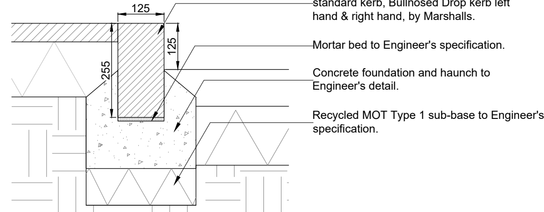
E4 Transition kerb - Left & right Scale: 1:10. Land. Spec.: Q10.111
