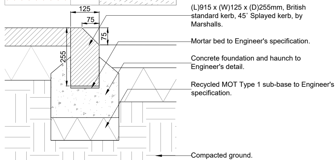
E8 45° Splayed kerb Scale: 1:10. Land. Spec.: Q10.114
