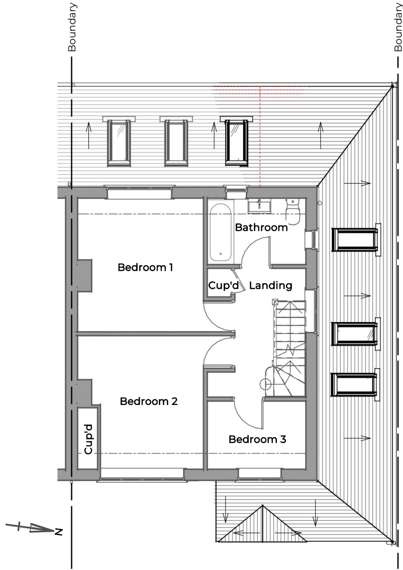
Proposed First Level Plan General Arrangement | Scale 1 : 100
