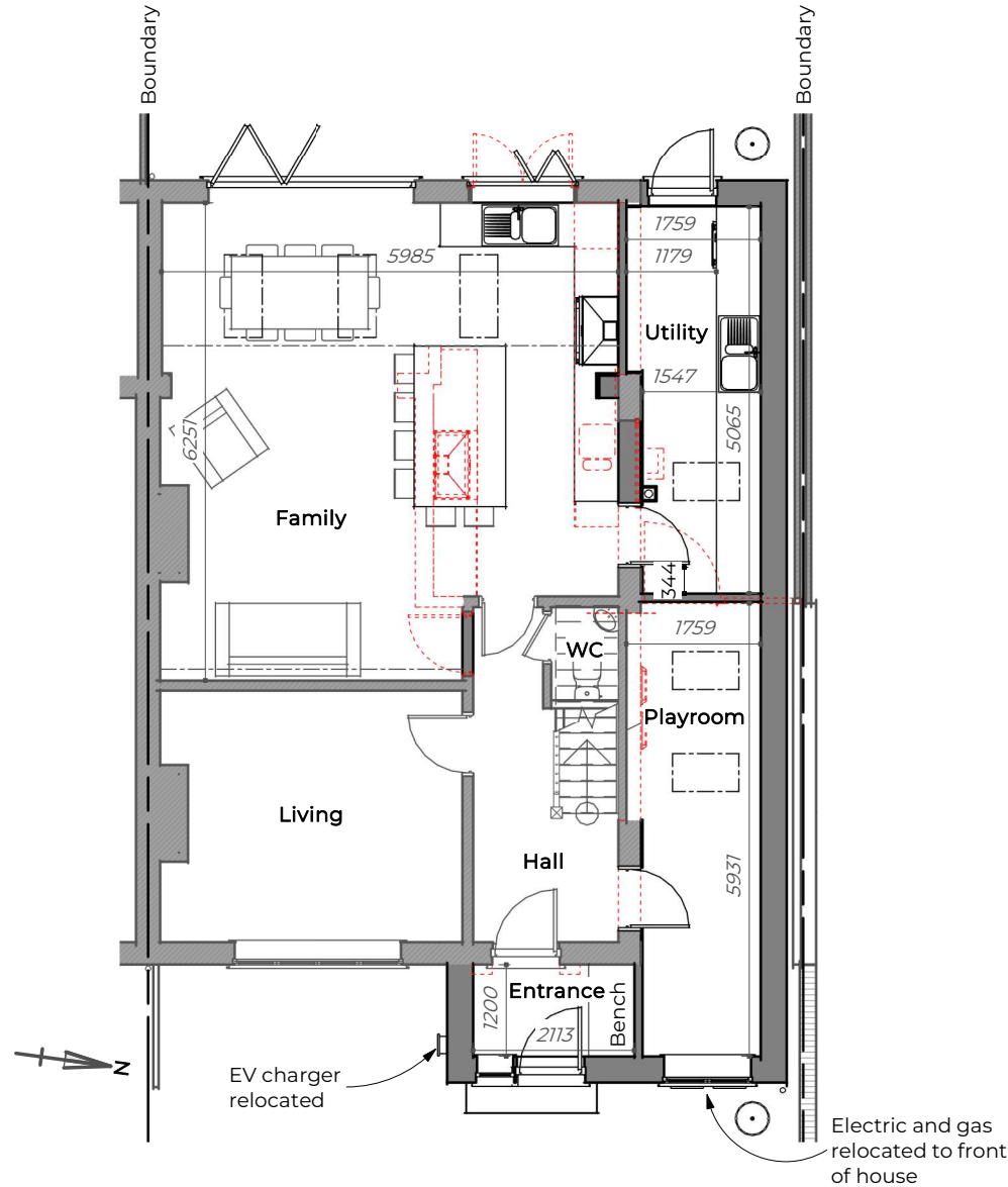
Proposed Ground Level Plan General Arrangement | Scale 1 : 100
