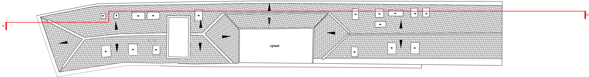
PROPOSED ROOF PLAN
