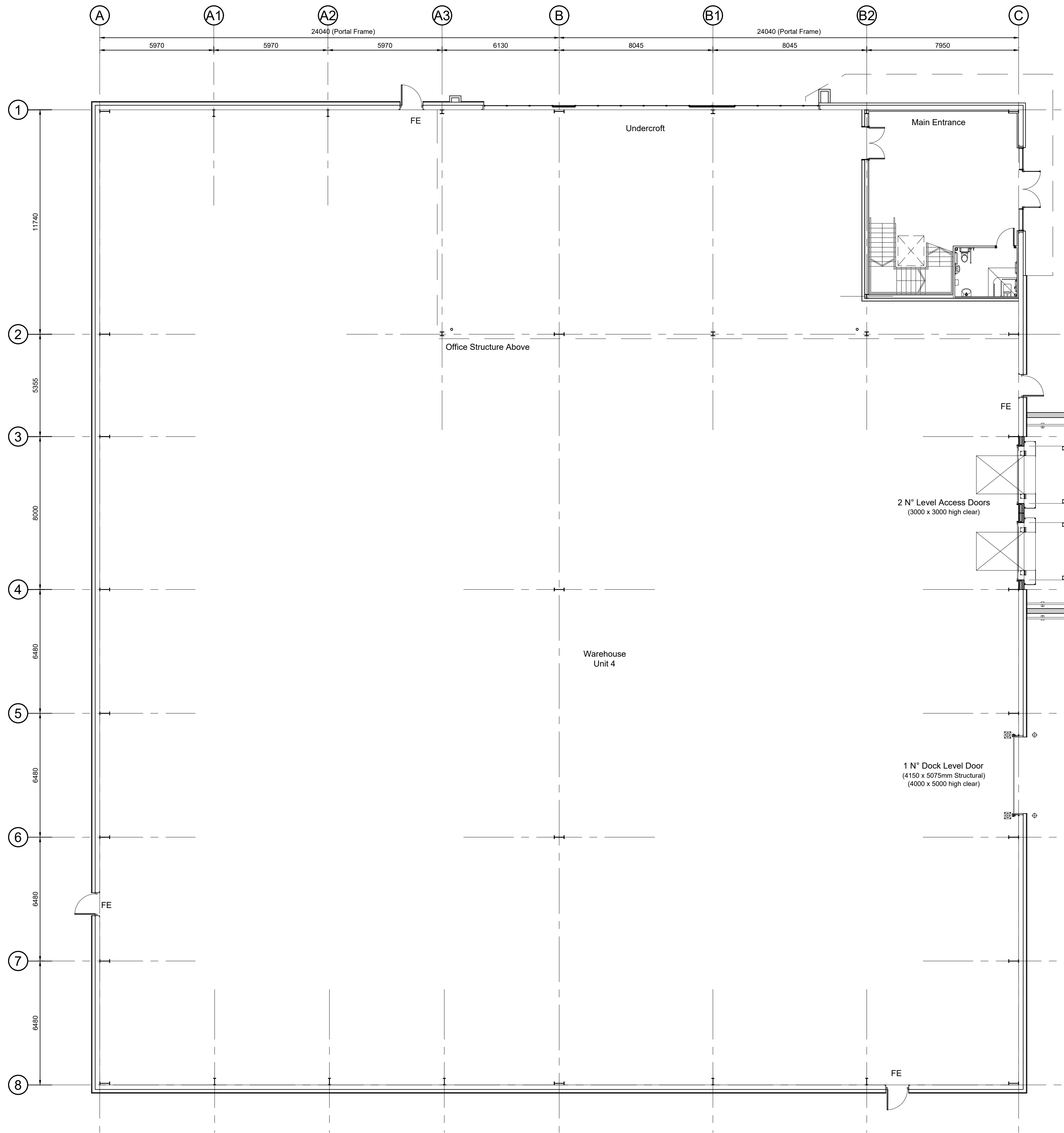
Ground Floor Warehouse Plan (0m FFL) - Scale 1:125
