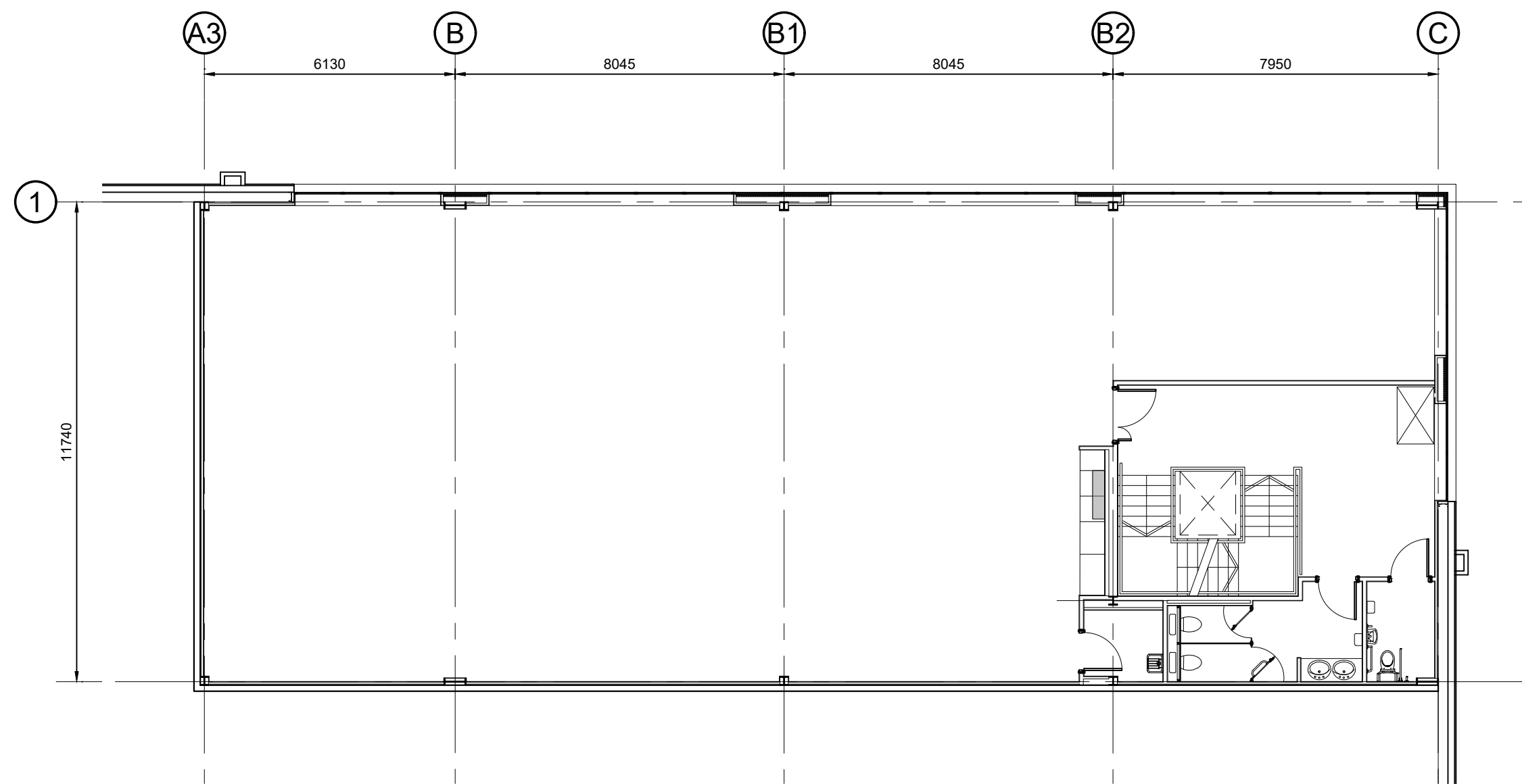
First Floor Office Plan (+4m FFL) - Scale 1:125
