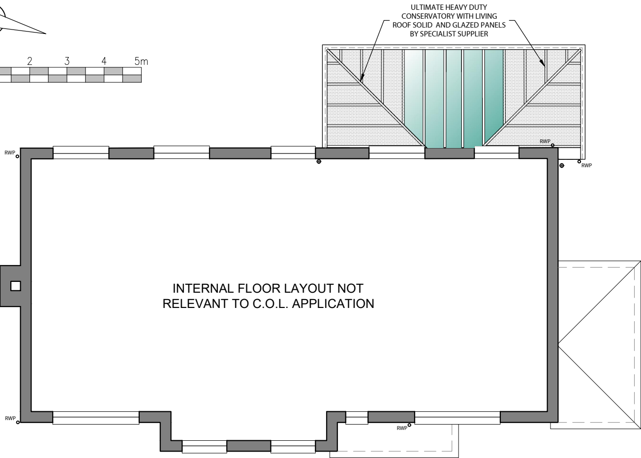
FIRST FLOOR PLAN AT 1:100
