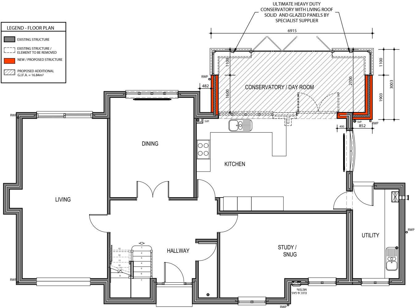
GROUND FLOOR PLAN AT 1:100
