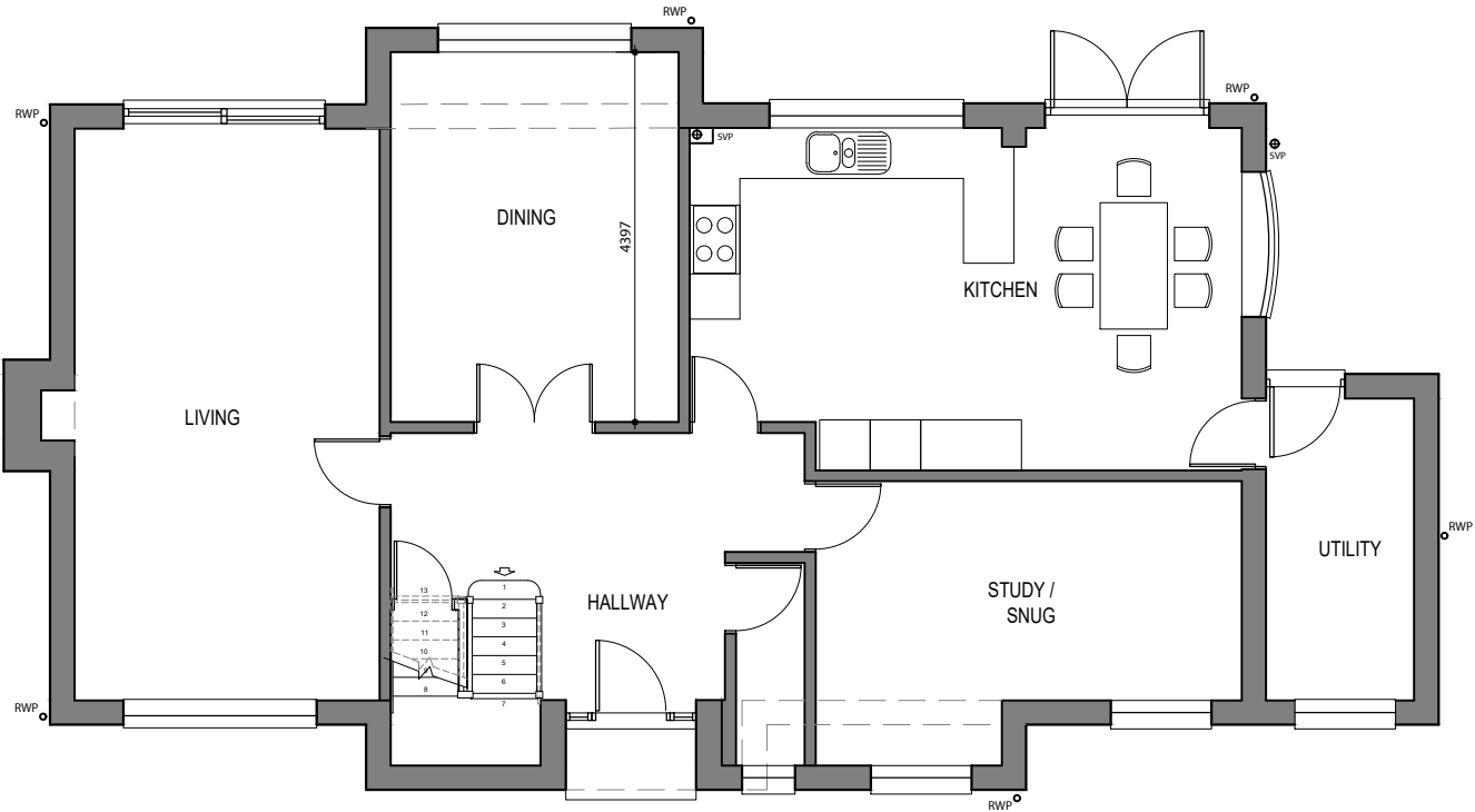
GROUND FLOOR PLAN AT 1:100
