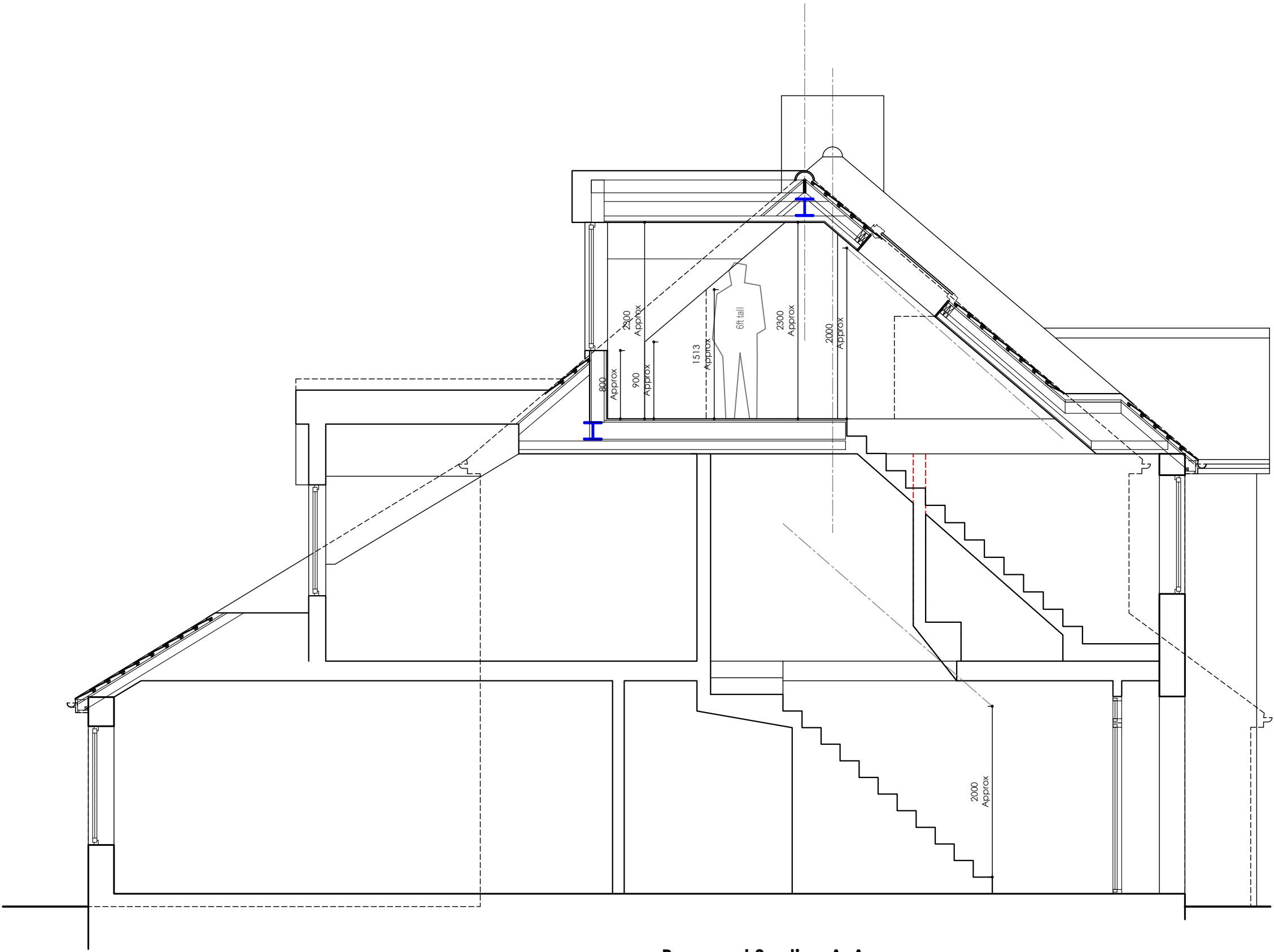
Proposed Section A-A Scale 1/50@A3
