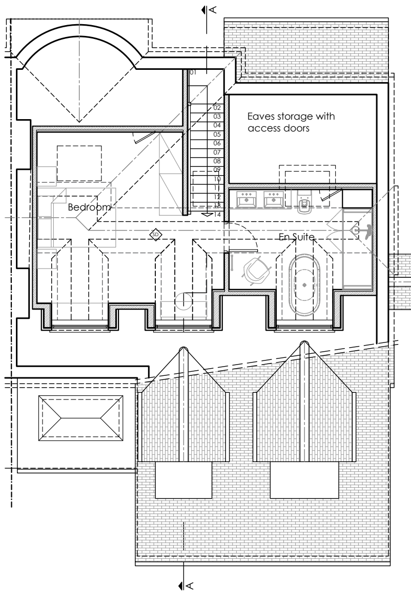
Proposed Second Floor Plan Scale 1/100@A3
