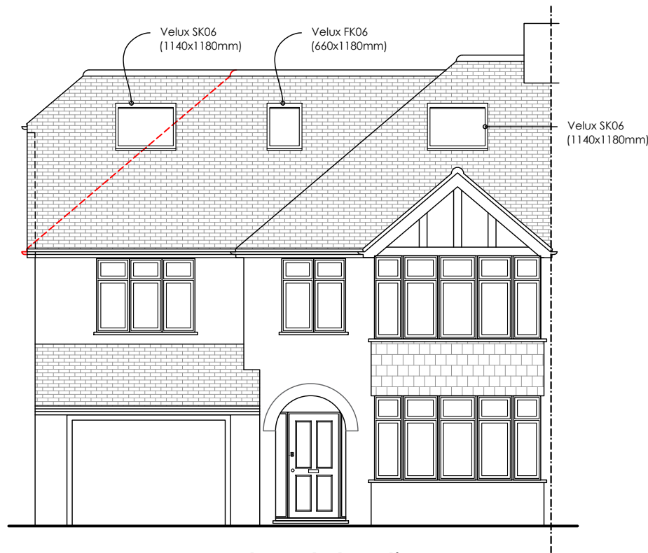
Proposed Front Elevation Scale 1/100@A3
