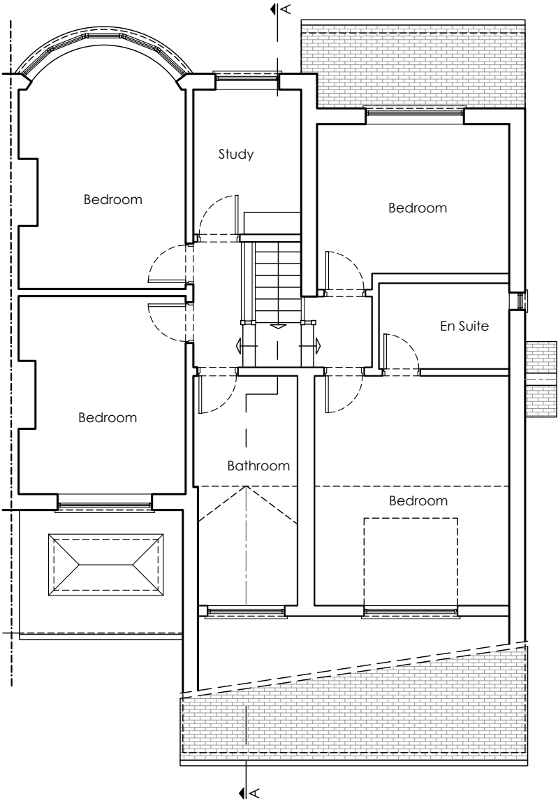
Existing First Floor Plan Scale 1/100@A3
