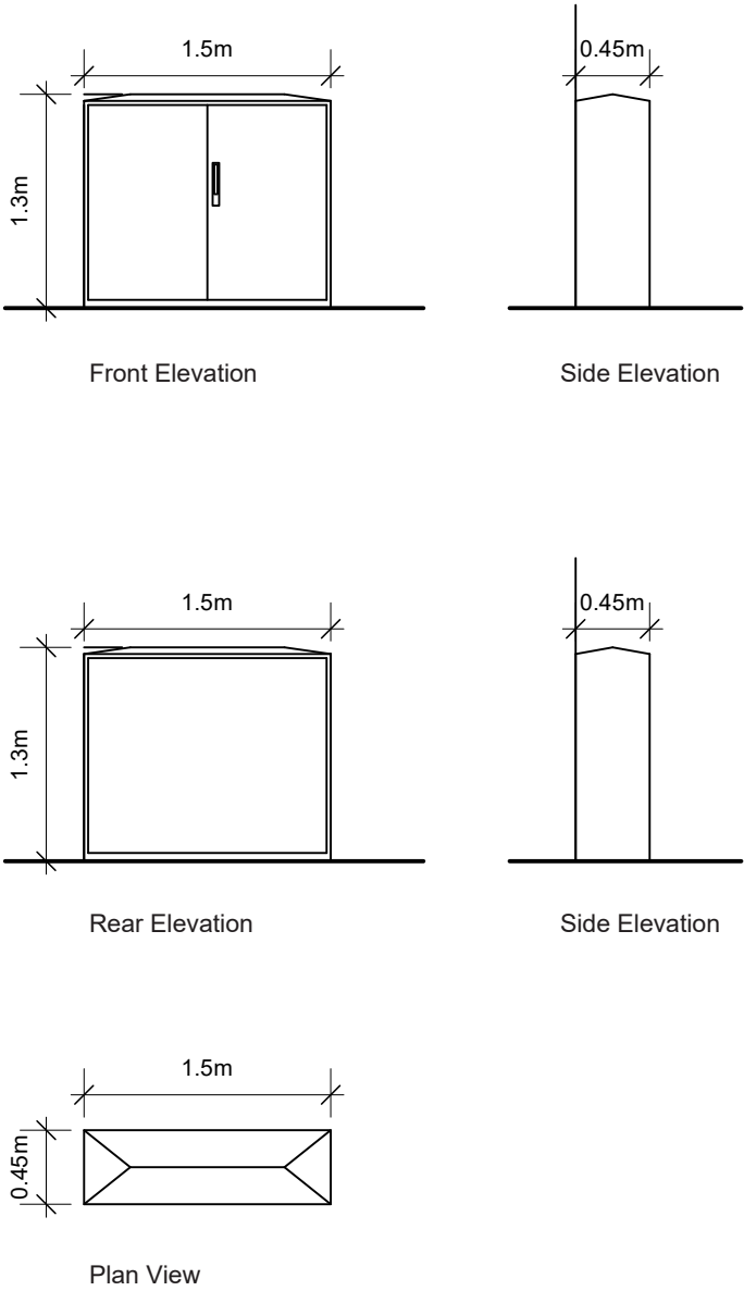
Electrical Cabinet
