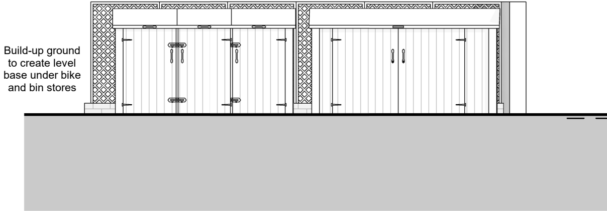
Bike & Bin Store Front - SW 1 : 50
