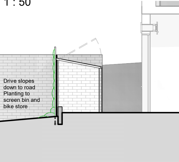
Bin Store Side - NW 1 : 50
