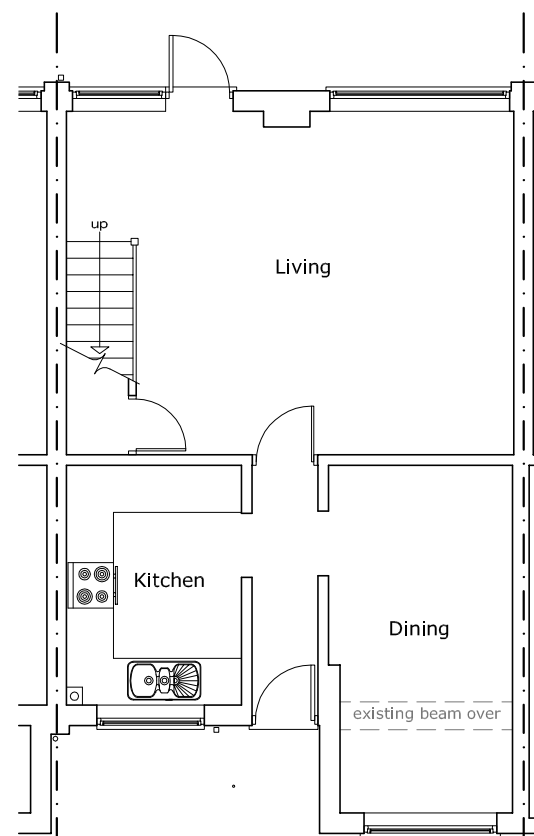
No. 18 No. 20 No. 22 Existing Ground Floor Plan
