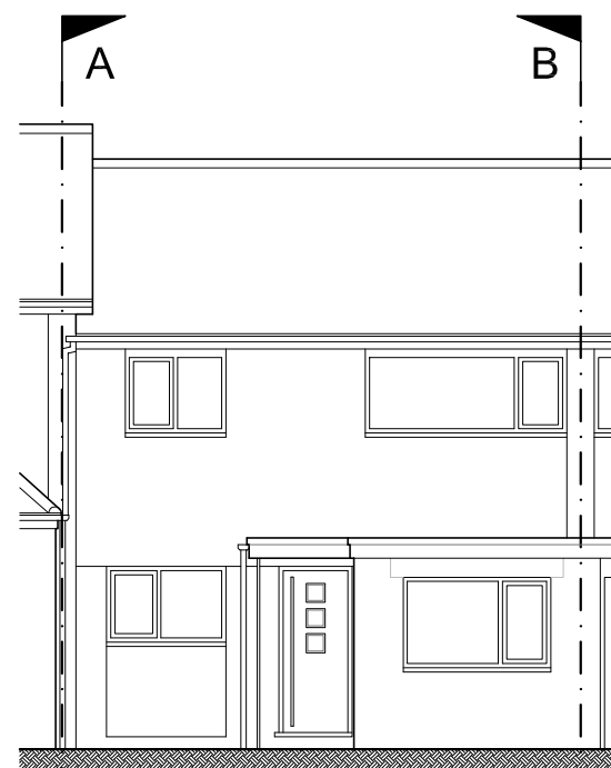
No. 18 A No. 20 B No. 22 Existing North (Front) Elevation
