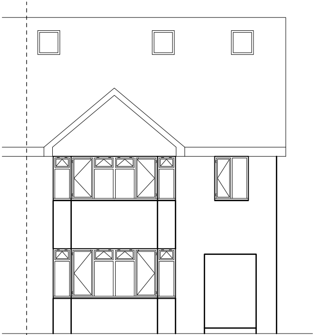
Proposed Front Elev
