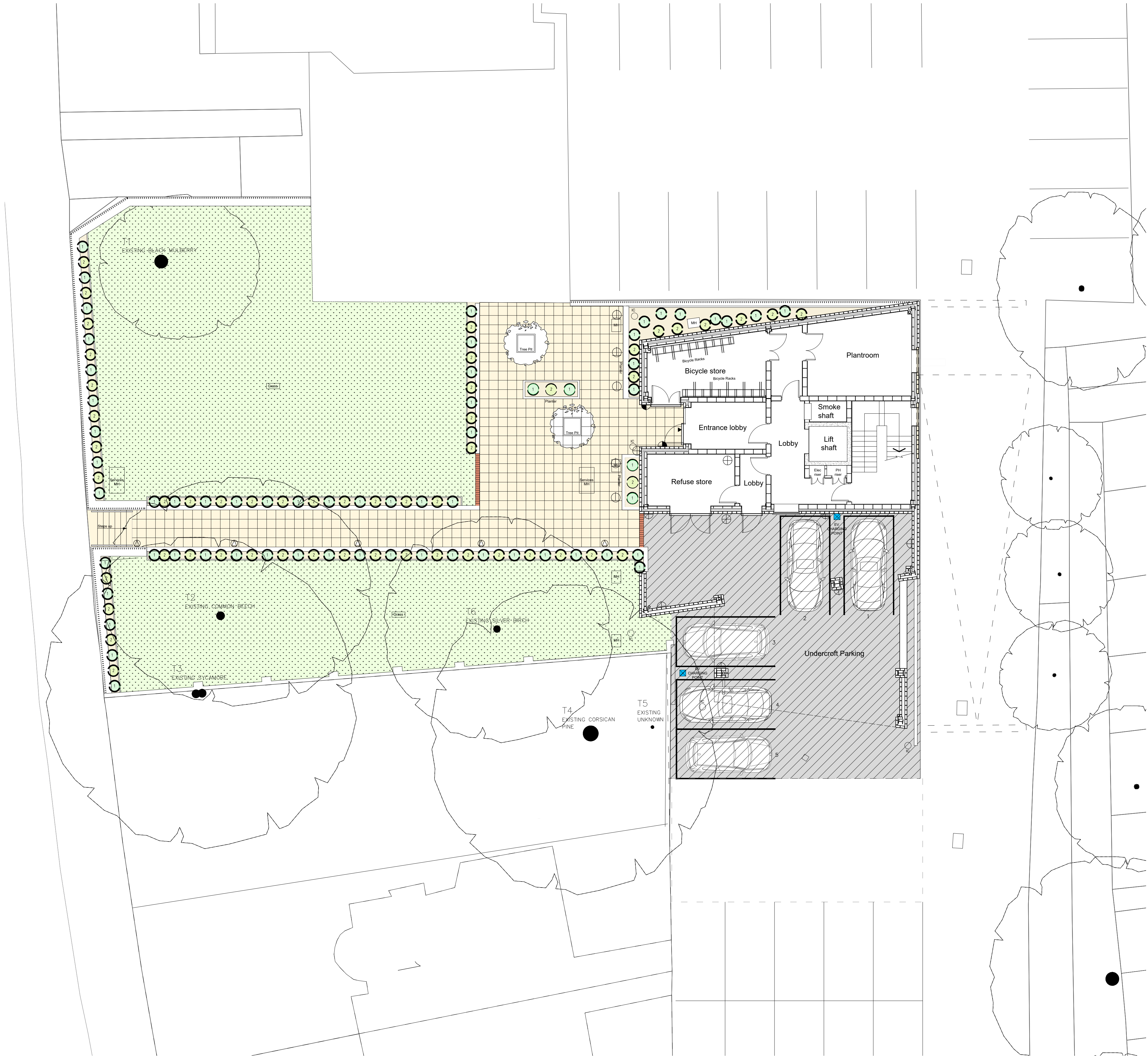
Proposed Landscaping Plan Scale 1:100
