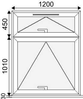
1 - 1200w x 1460h (Basic Frame Size) 1 - 1200w x 1490h, 30mm Cill Viewed Outside Style No: 111
