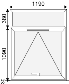
1 - 1190w x 1470h (Basic Frame Size) 1 - 1190w x 1500h, 30mm Cill Viewed Outside Style No: 107
