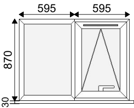
1 - 1190w x 870h (Basic Frame Size) 1 - 1190w x 900h, 30mm Cill Viewed Outside Style No: 206
