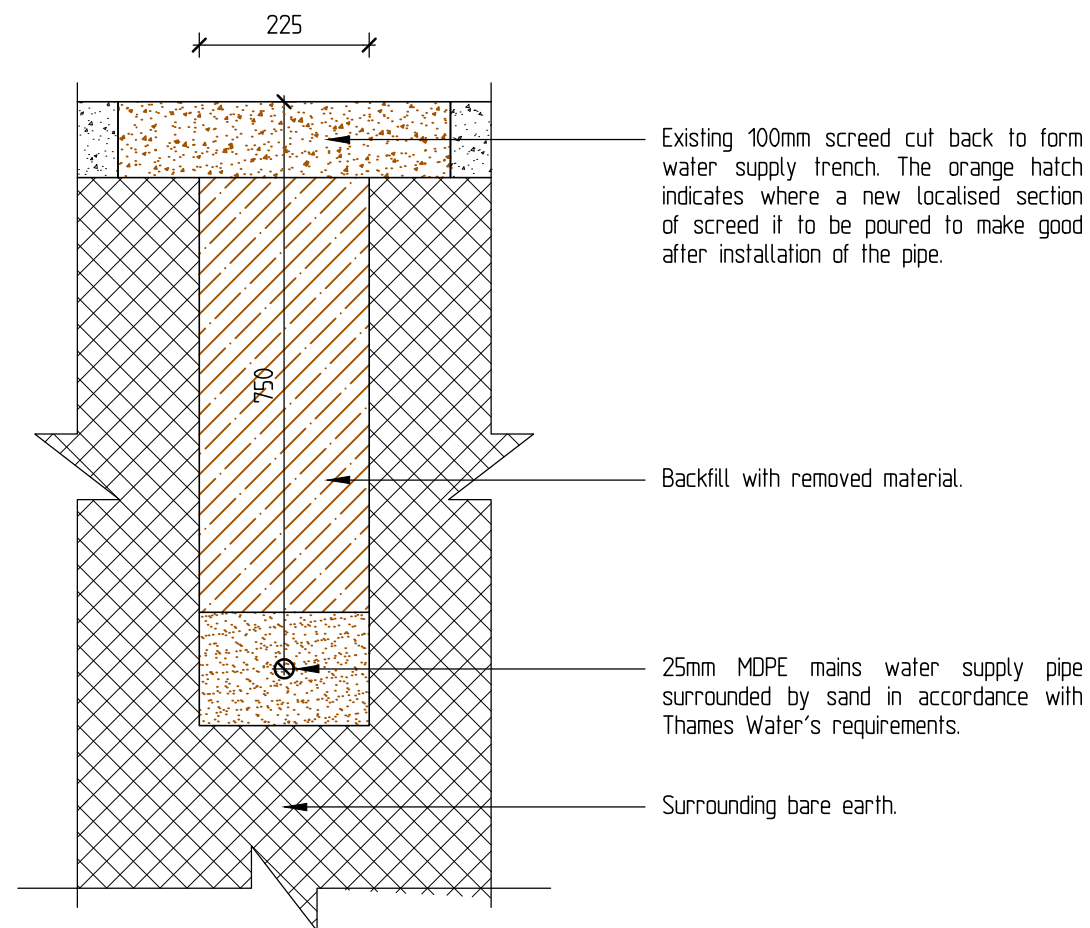
Detail B - Kitchen Floor
