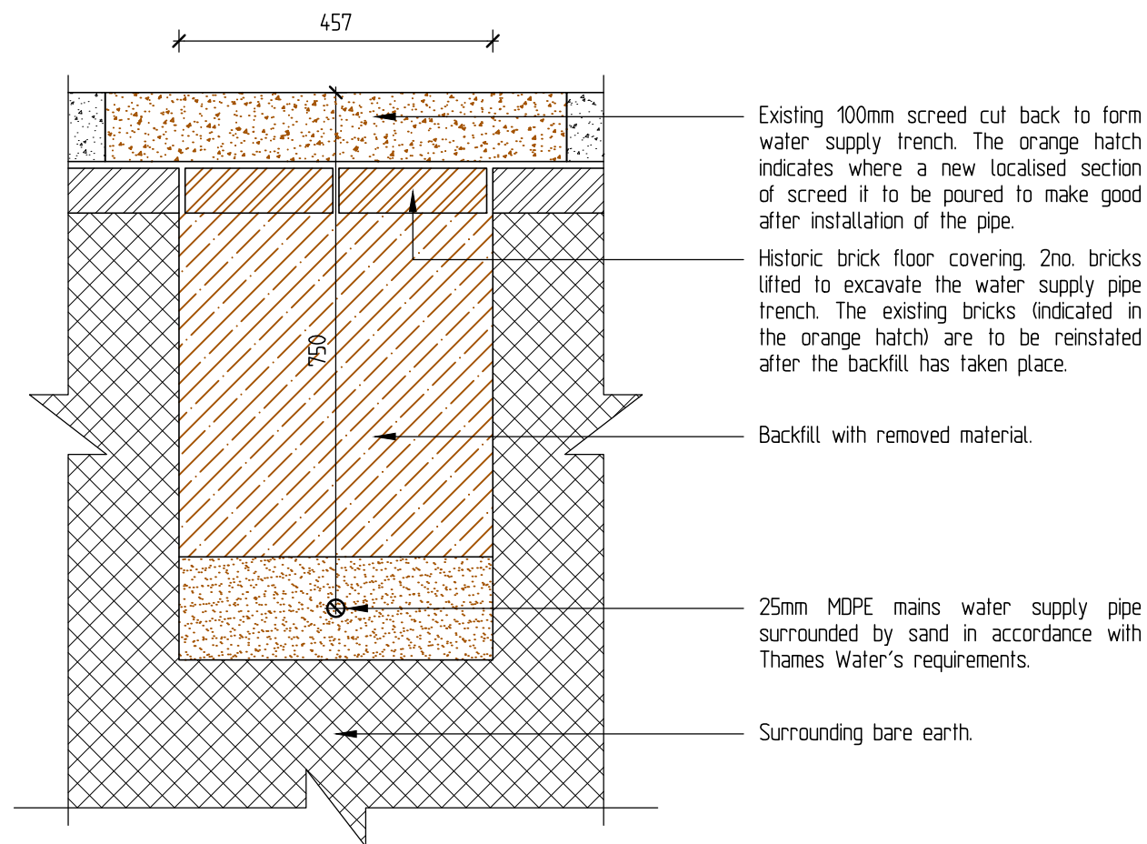
Detail A - Dining Room Floor
