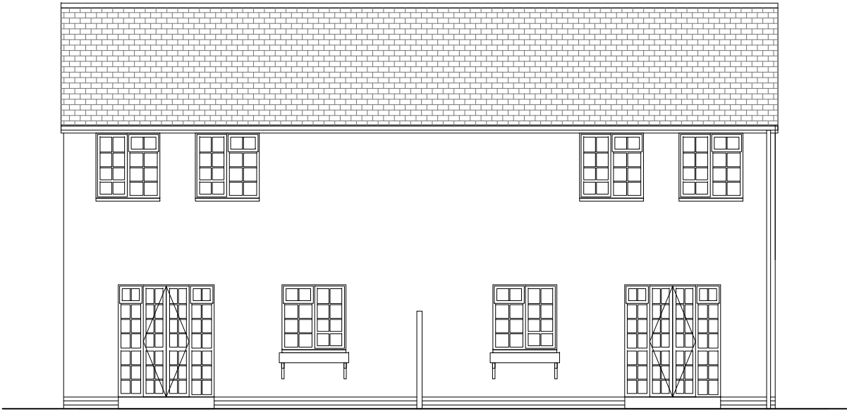
01 PROPOSED REAR - NORTH ELEVATION 1:100
