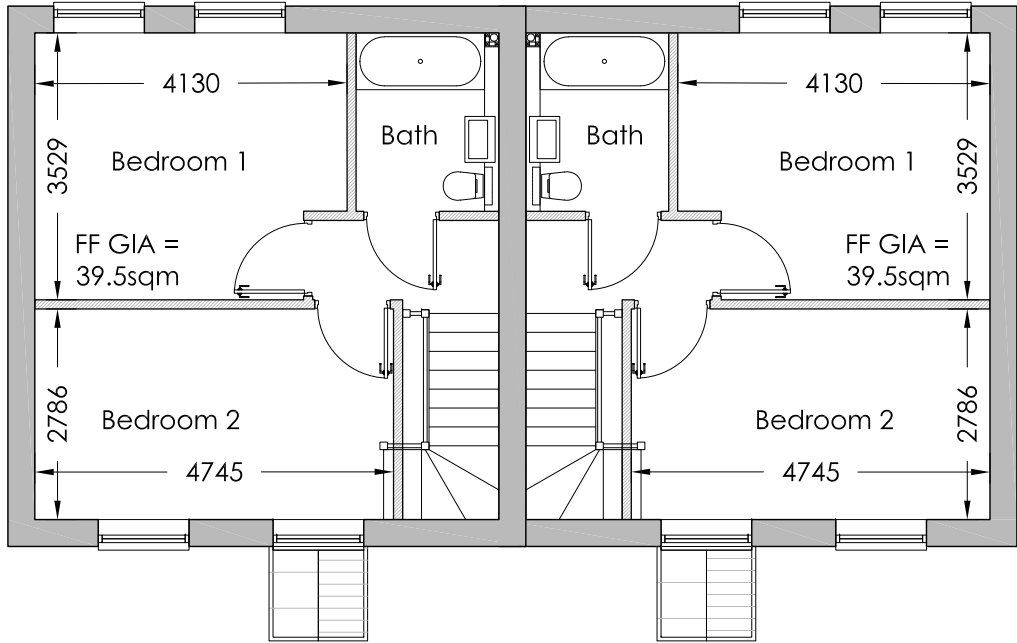
01 PROPOSED FIRST FLOOR PLAN 1:100
