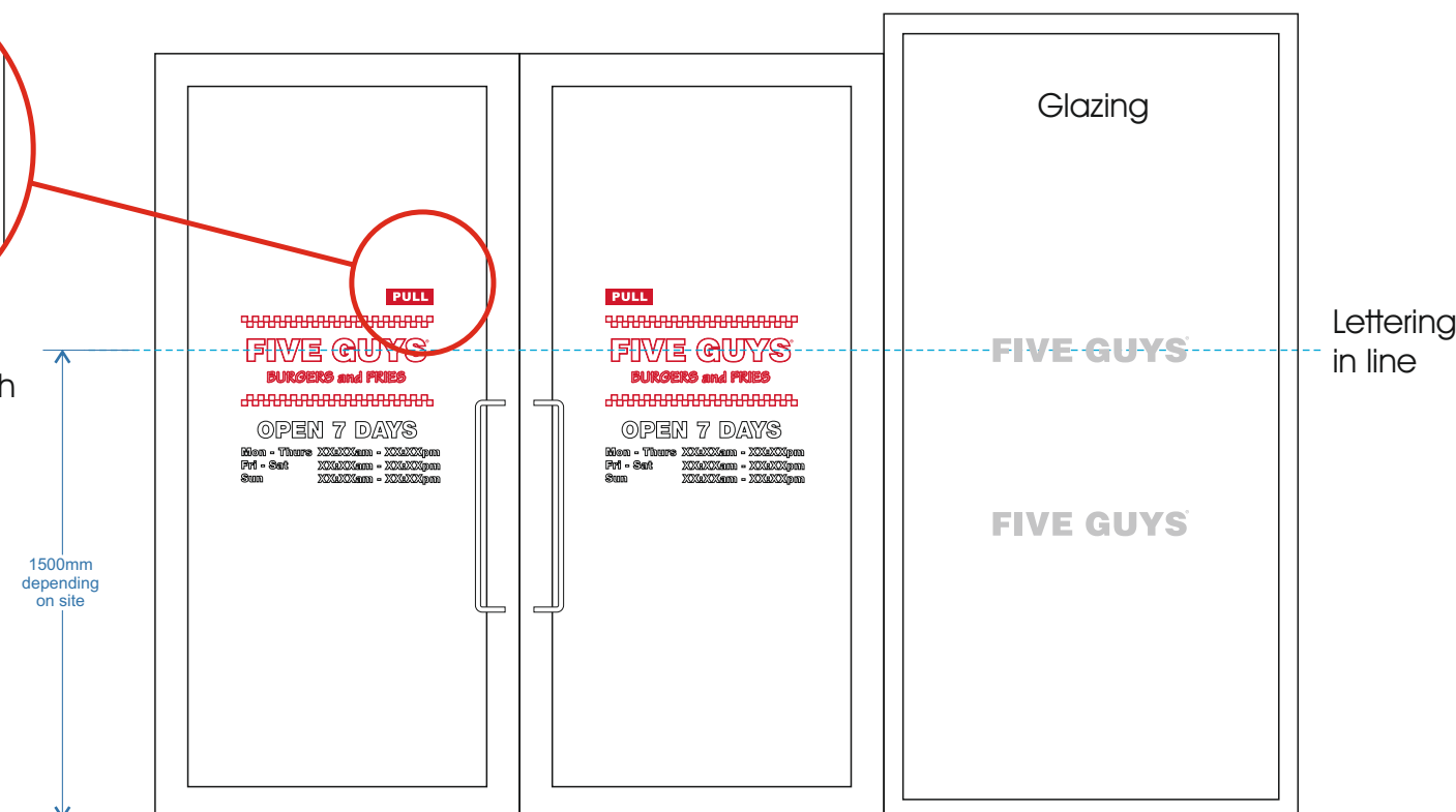
Example Layout Scale 1:25
