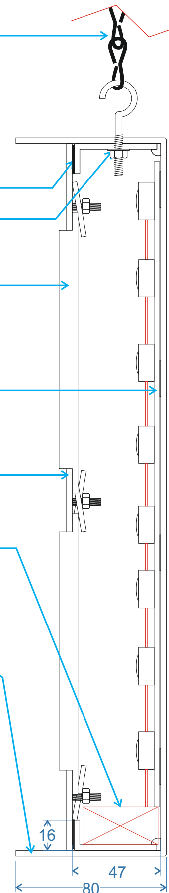
Sign Section Scale 1:2
