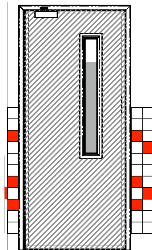
Scale 1:20 Frosted vinyl panel to glazing. Starting 200mm from top.
