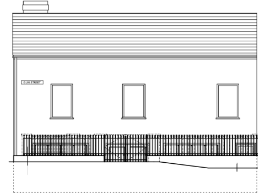
Front Elevation (street)
