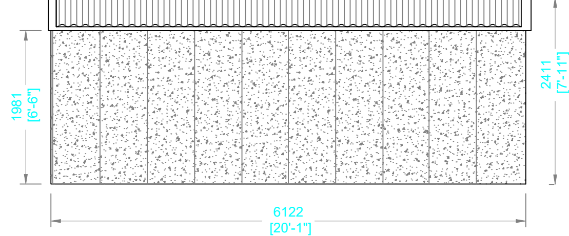
FRONT ELEVATION
