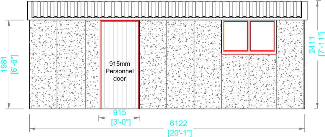
RH ELEVATION
