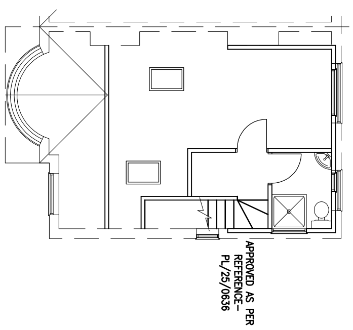
PROPOSED LOFT FLOOR PLAN
