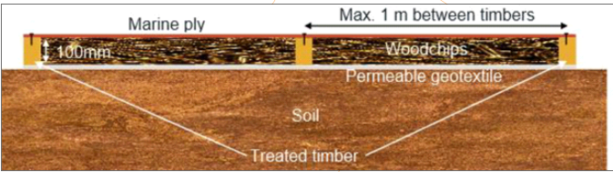
Ground protection
