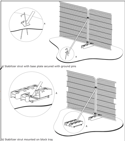
Protective fencing
