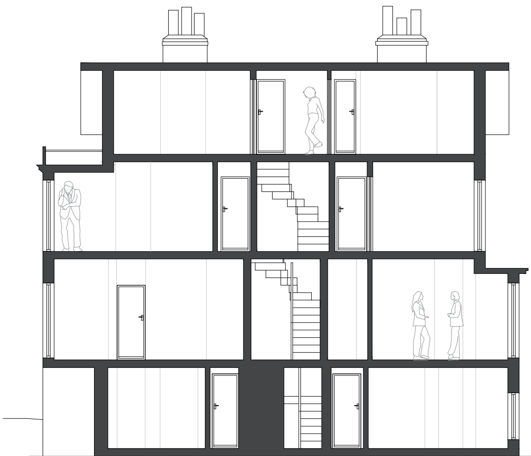
PROPOSED SECTION (BB) 1:100
