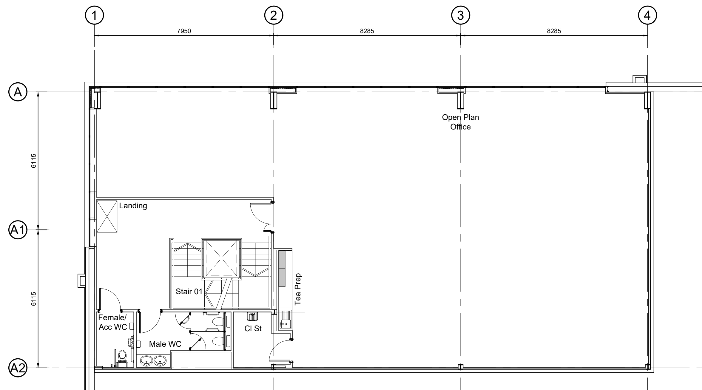
First Floor Main Office Plan (+4m FFL) - Scale 1:100
