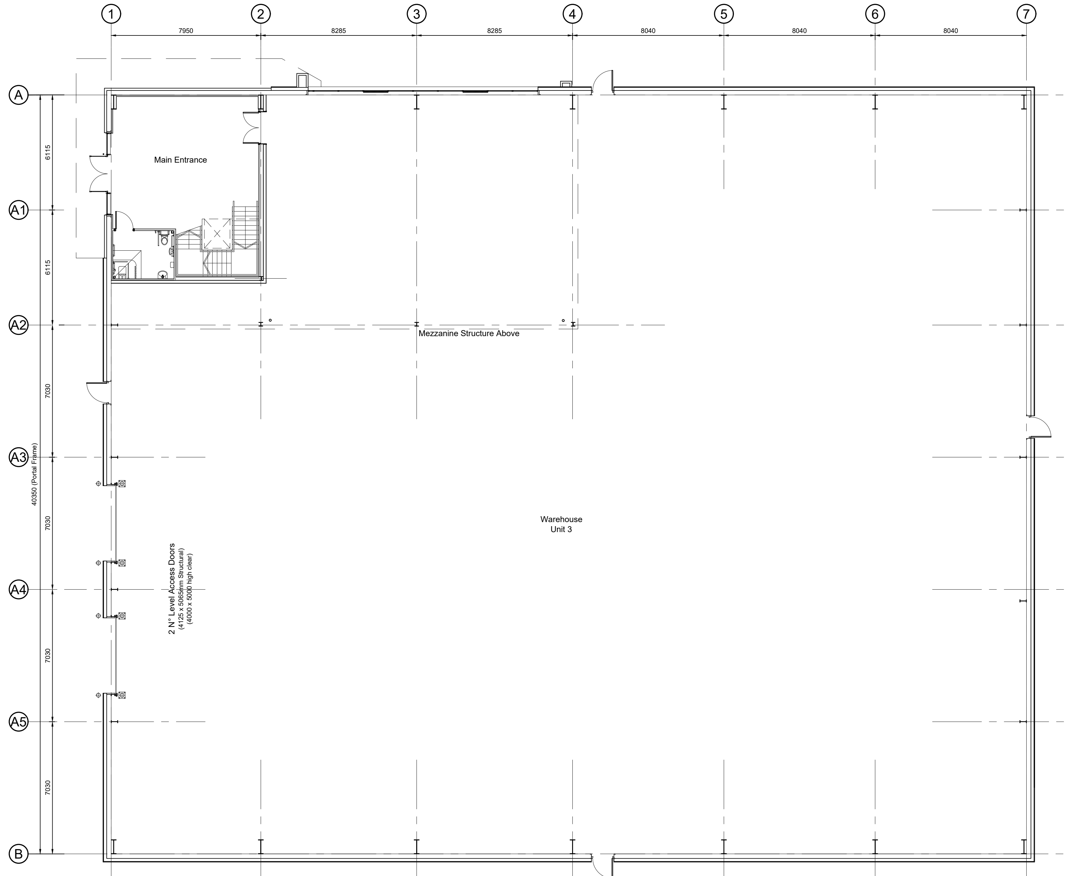
Warehouse Plan - Scale 1:125
