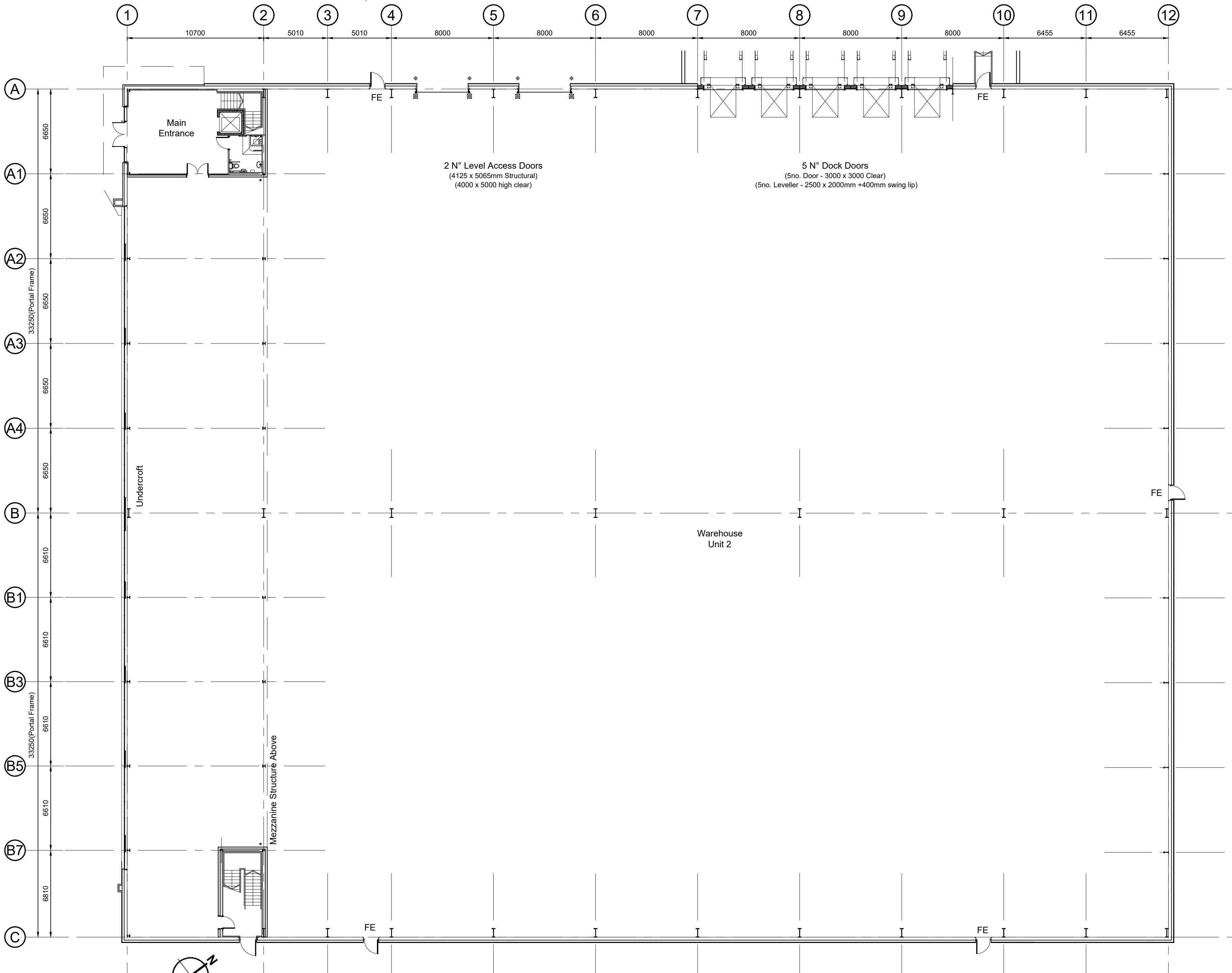
Ground Floor Layout Scale 1:200
