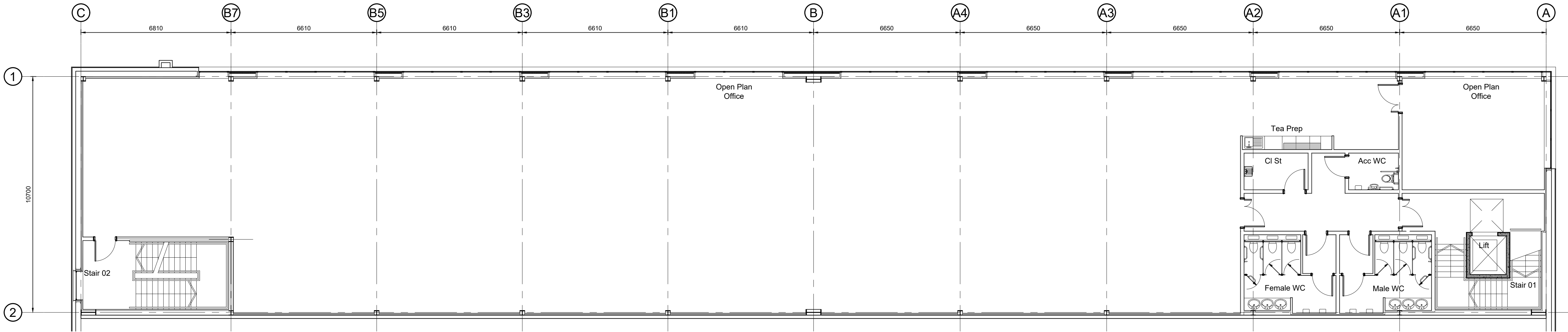
First Floor Office Plan (+4m FFL) - Scale 1:100
