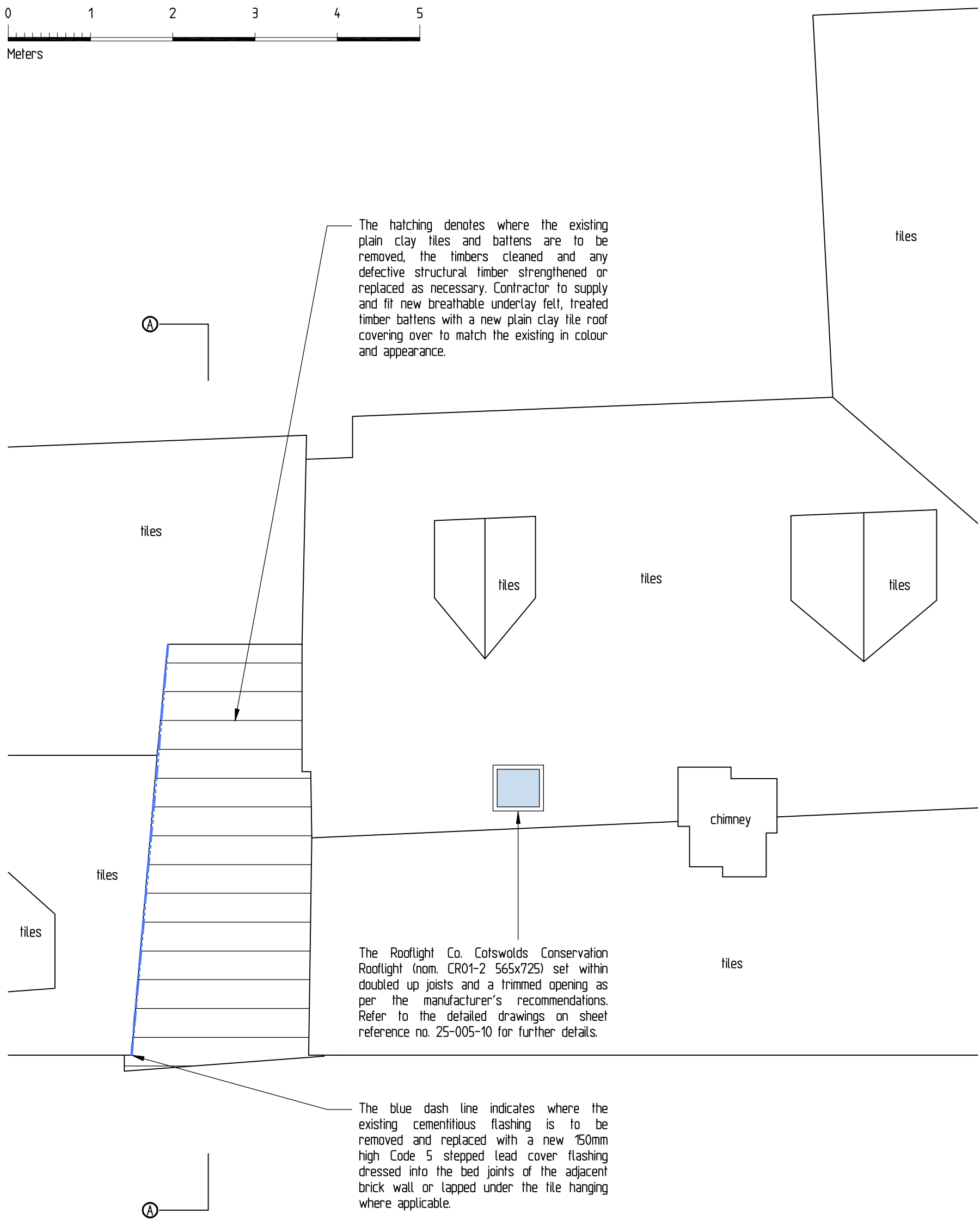
Roof Plan - 1:50
