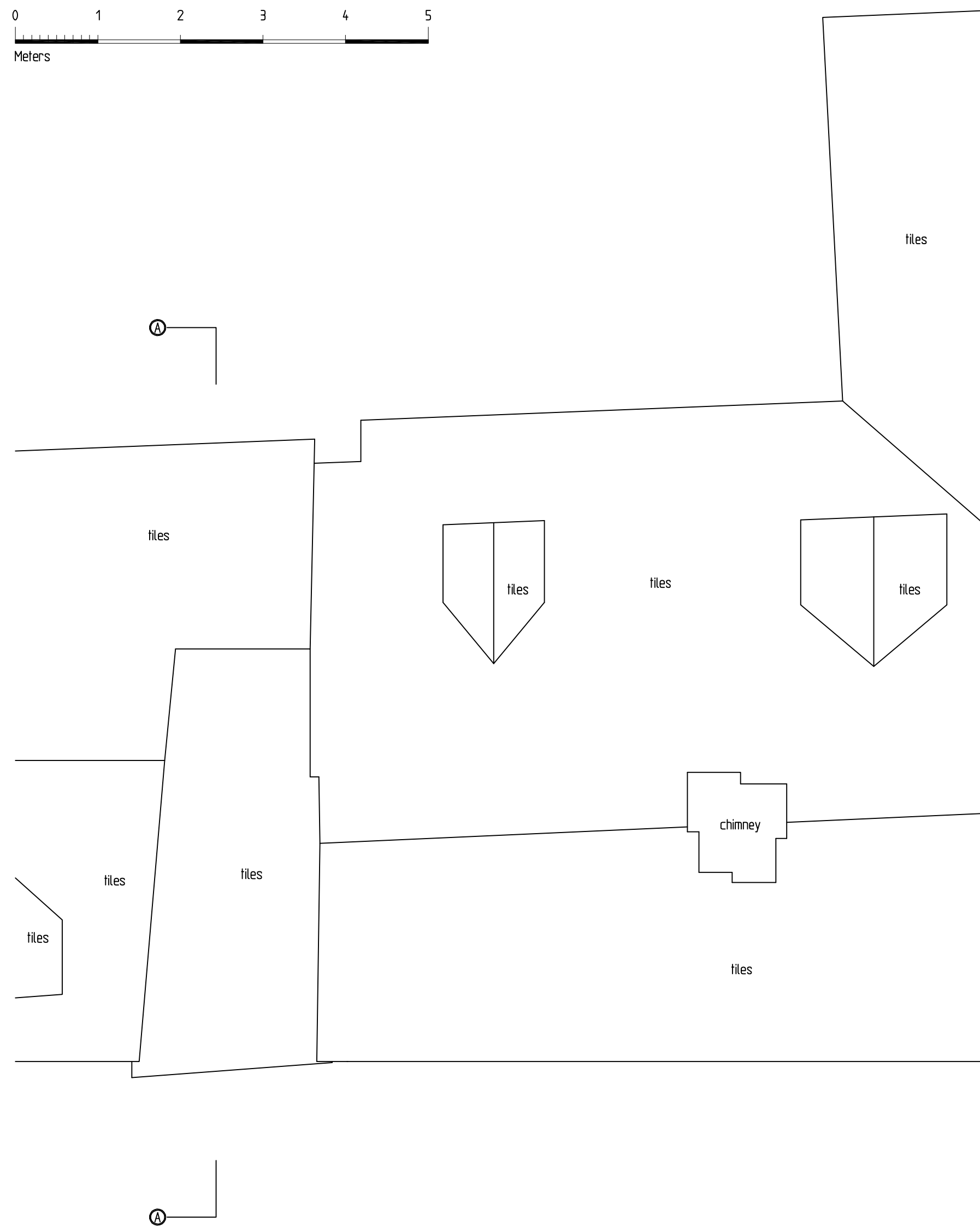
Roof Plan - 1:50
