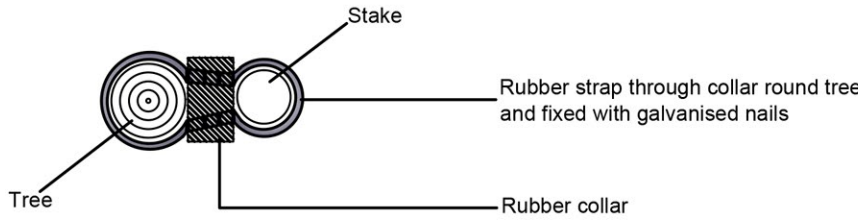
Tree Pit detail NTS
