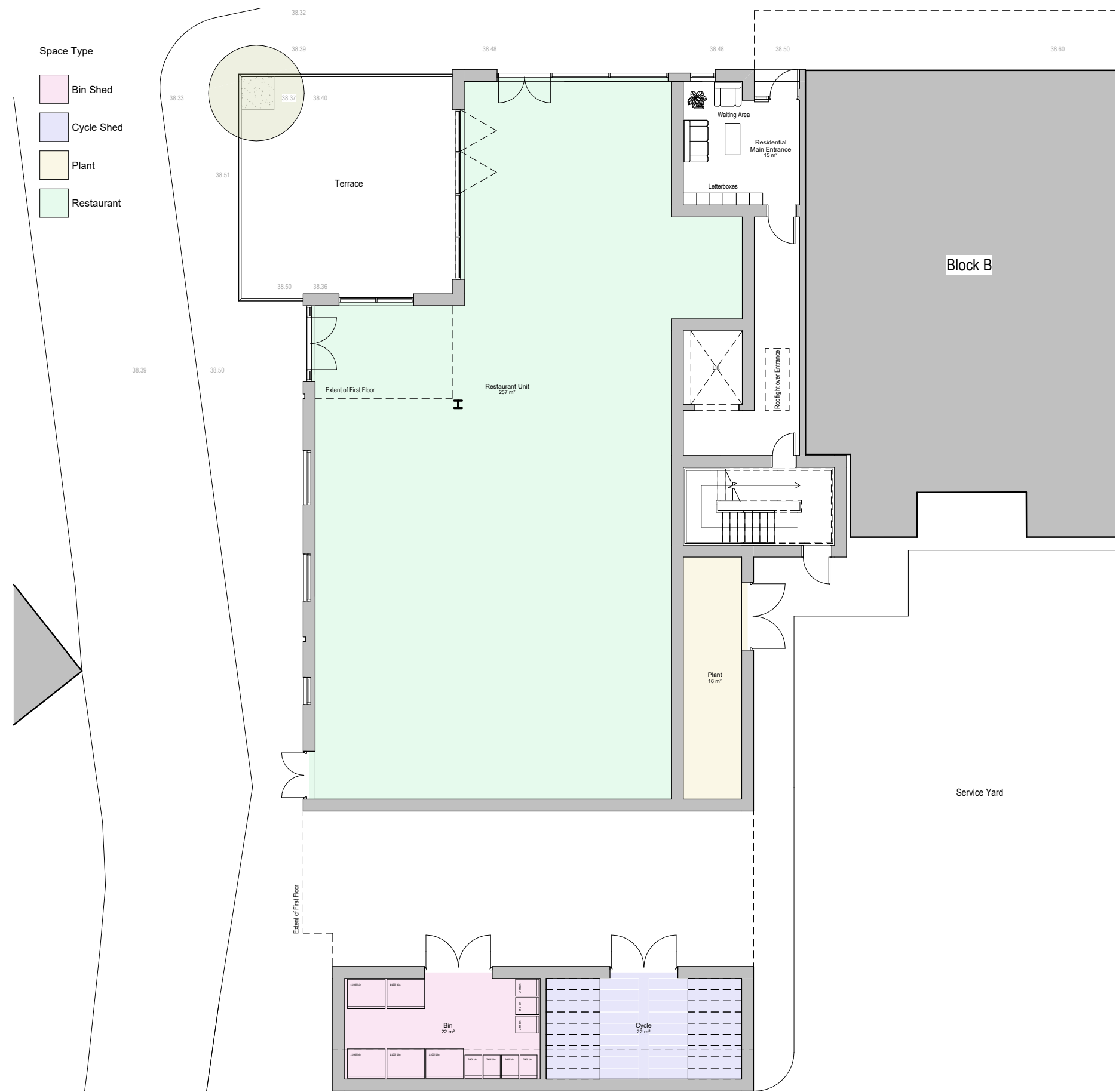
Block A - Proposed Ground Floor Plan
