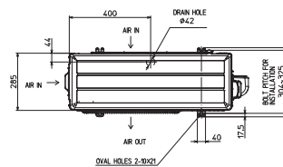
Upper View
