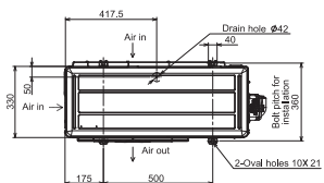
Upper View
