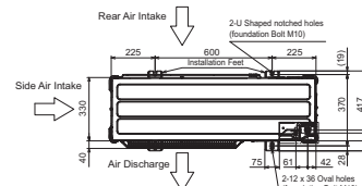
Upper View
