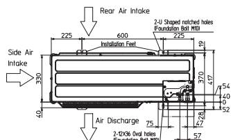
Upper View
