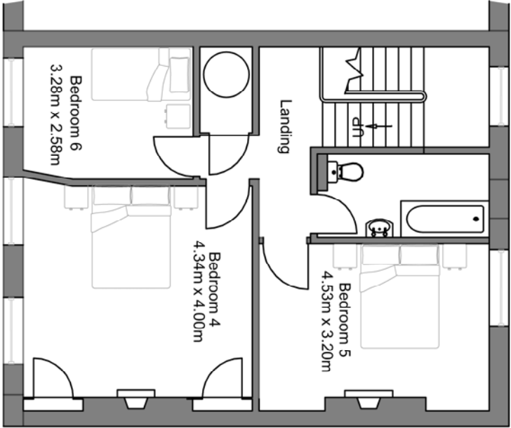
Existing & Proposed Second Floor
