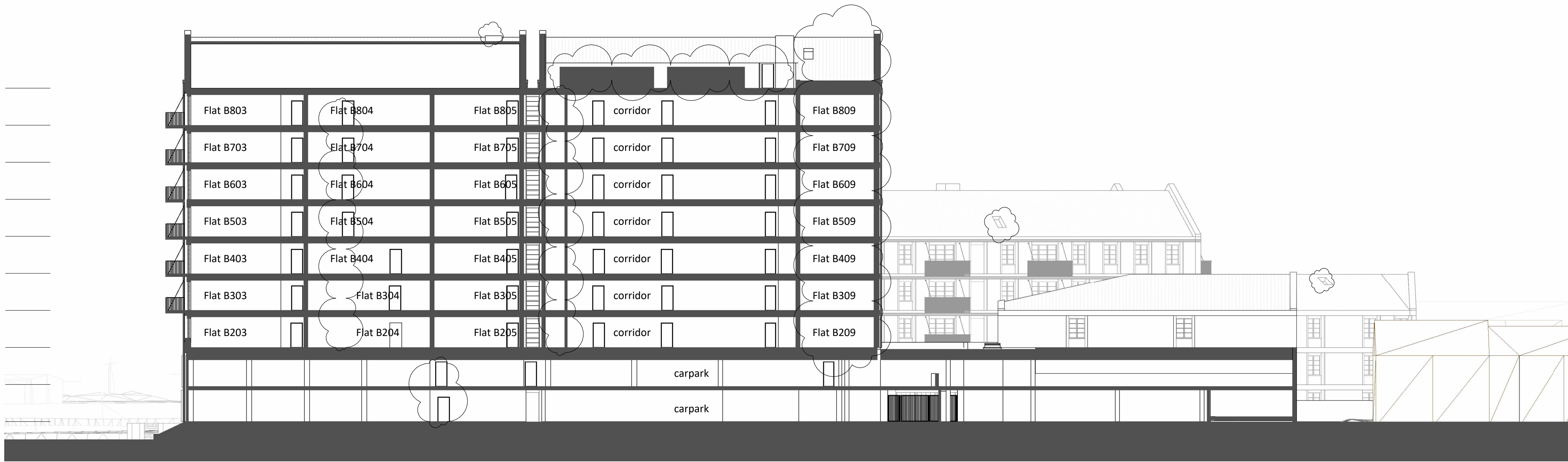
1 Proposed section 1 : 250
