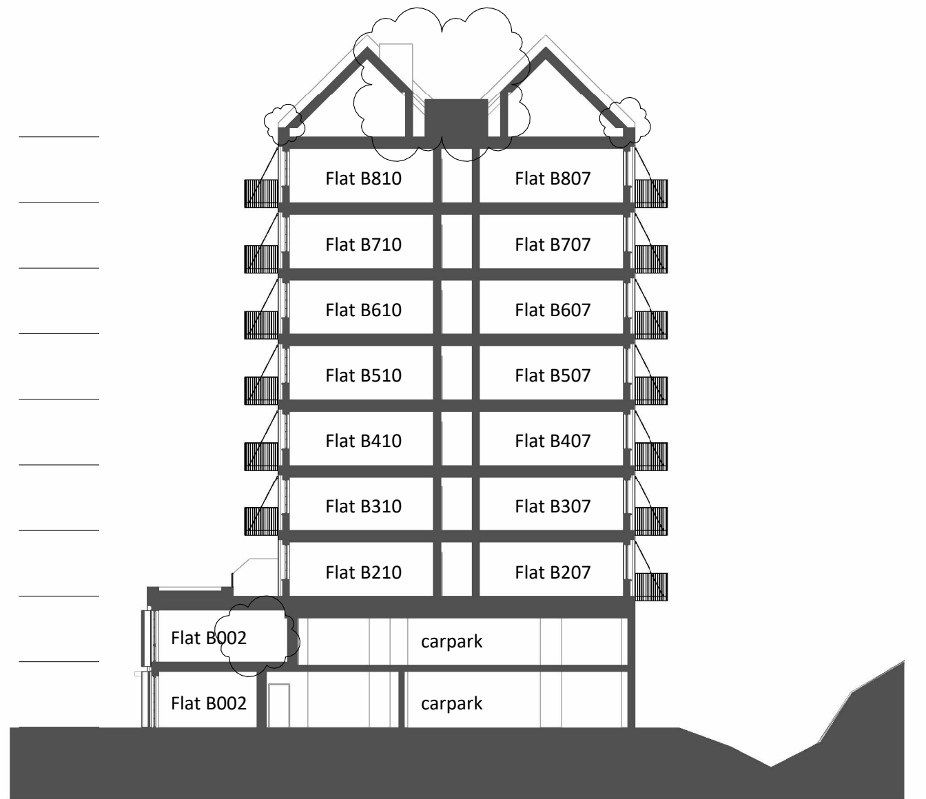
2 Proposed section 1 : 250
