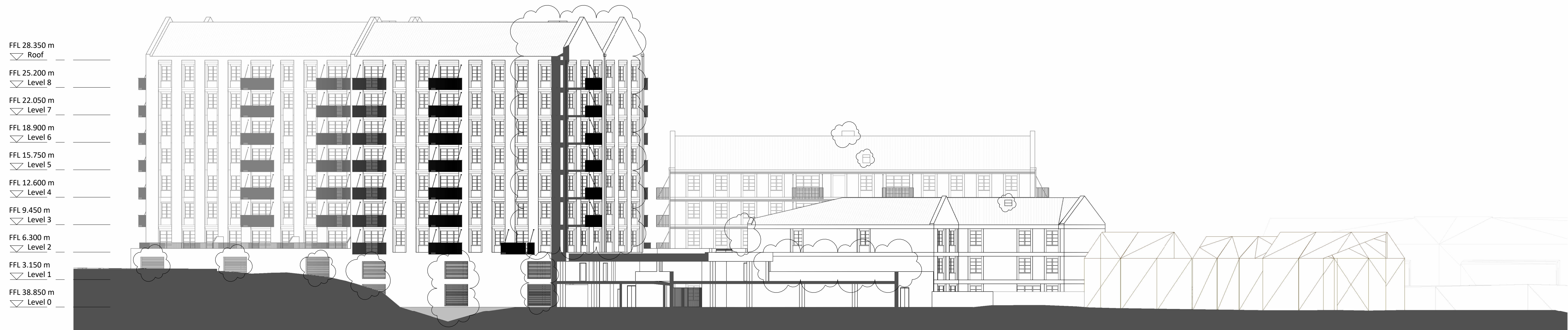
2 Proposed North Context Elevation 1 : 250
