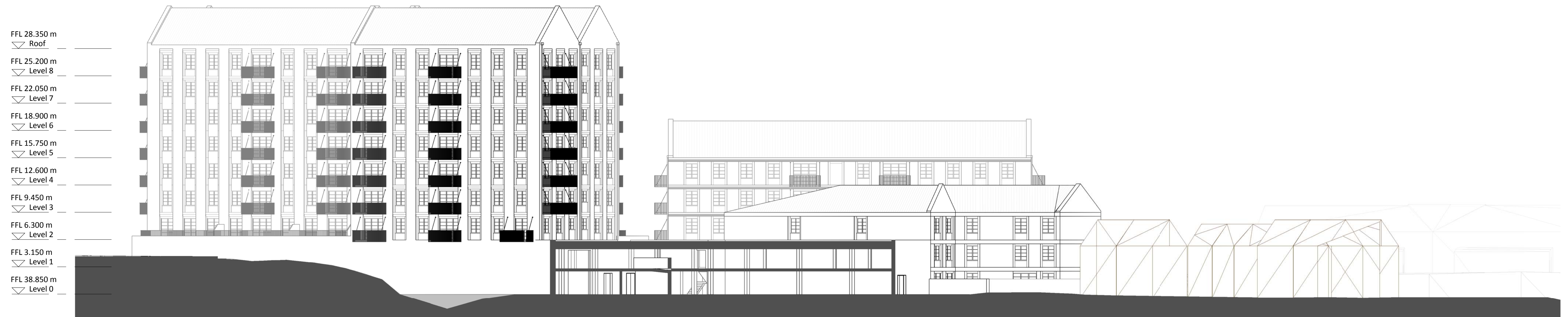
2 Proposed North Context Elevation 1 : 250
