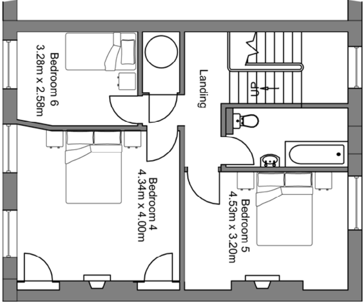
Existing & Proposed Second Floor
