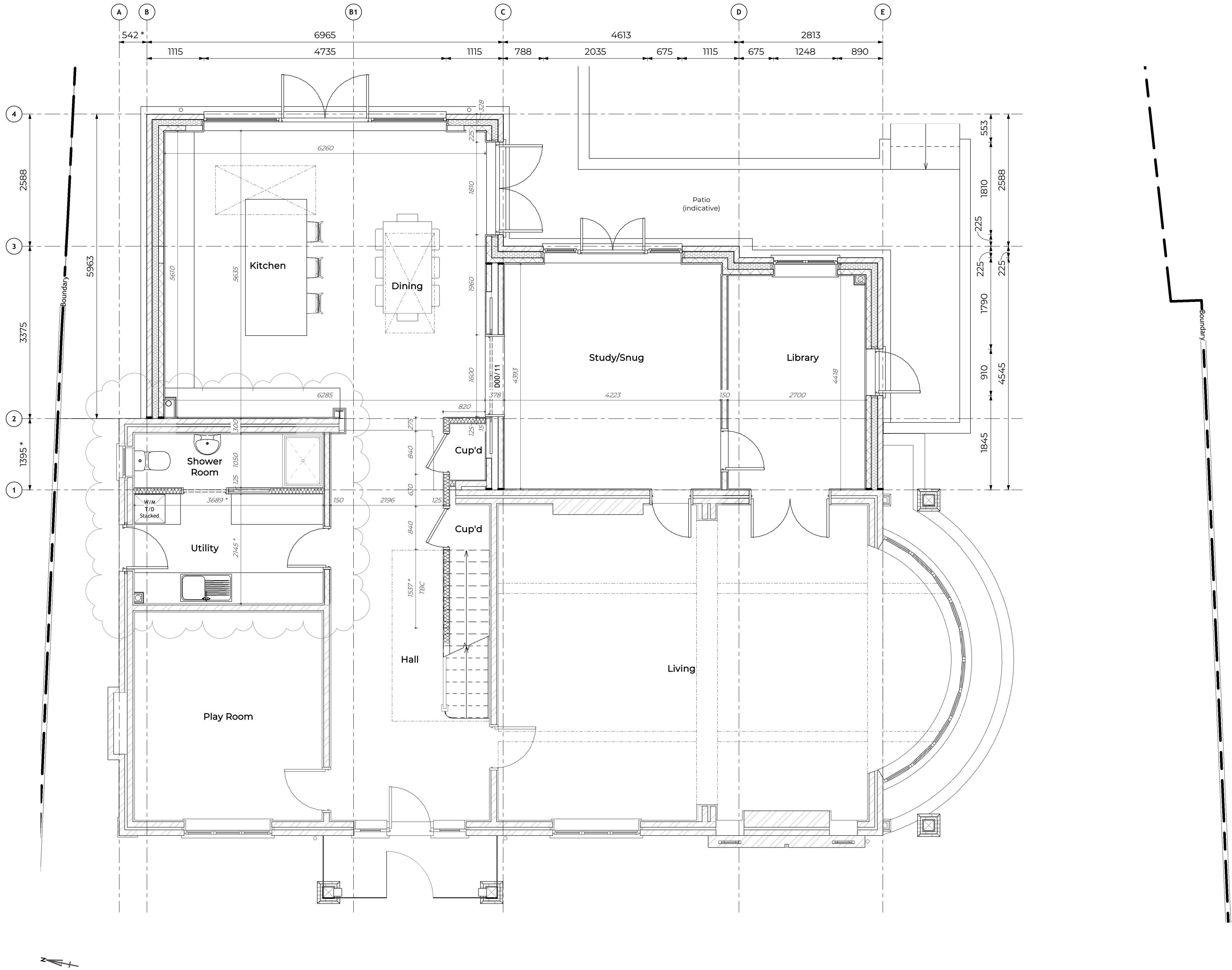
Proposed Site Level Plan General Arrangement | Scale 1 : 50
