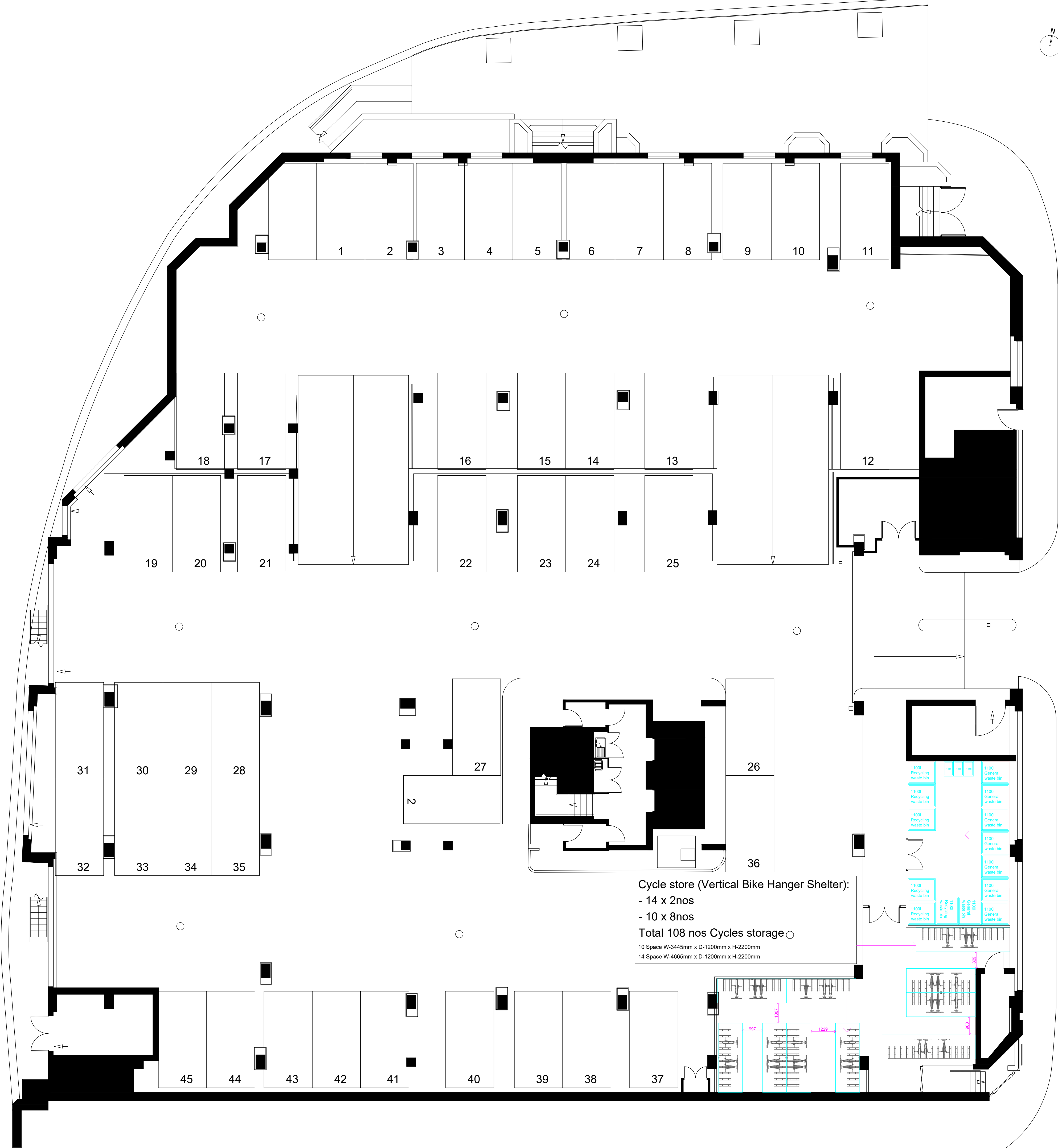
PROPOSED BASEMENT FLOOR
