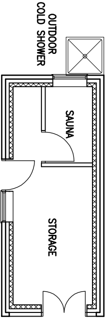
PROPOSED GARAGE FLOOR PLAN
