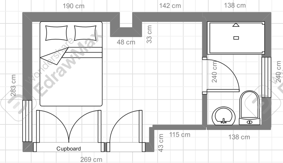
Current Floor Plan
