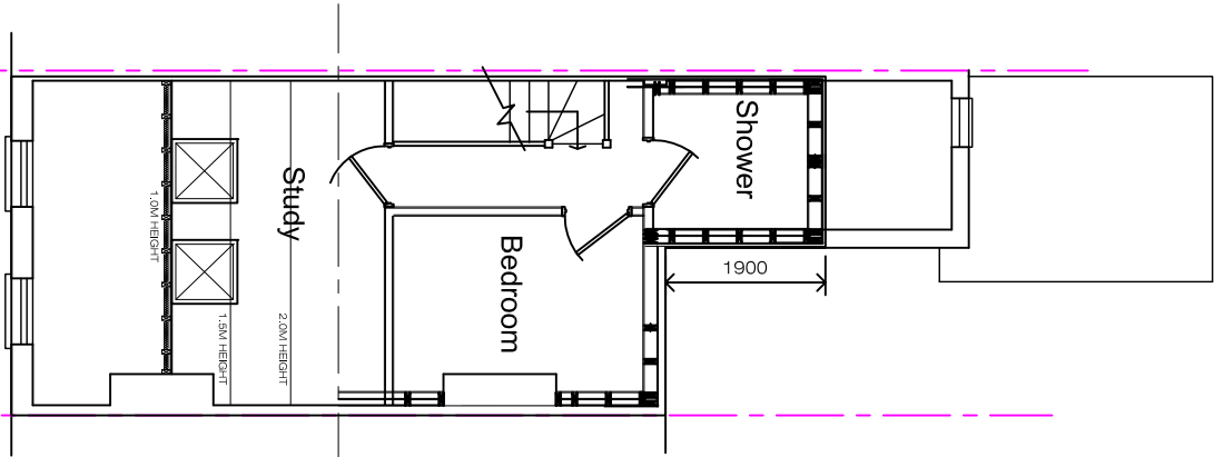
Loft Floor Plan
