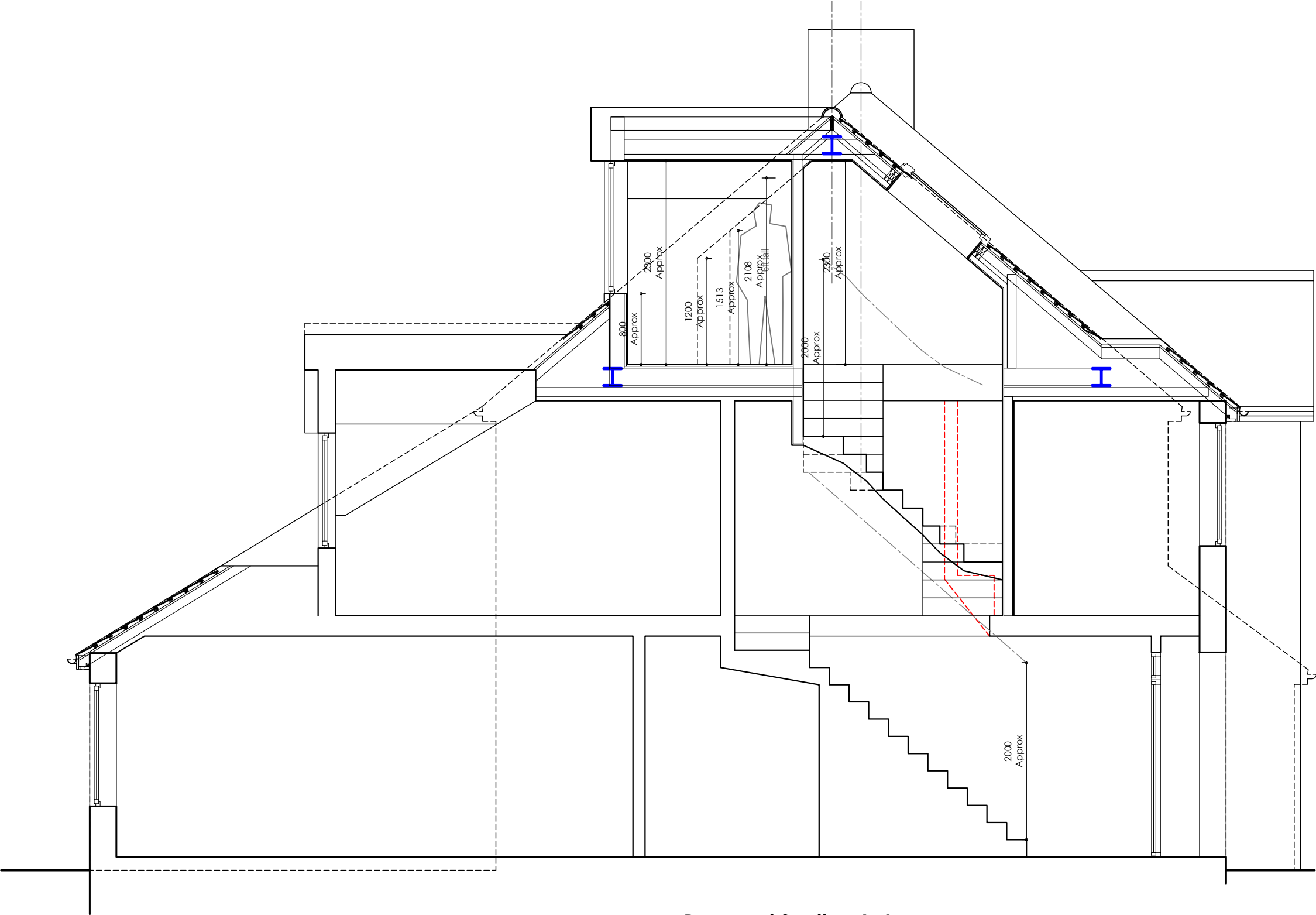
Proposed Section A-A Scale 1/50@A3
