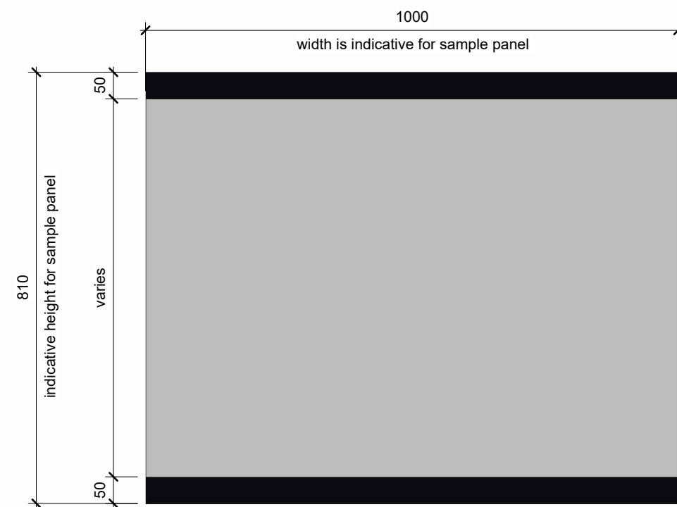
Railing type 6 Glass balustrade with handrail height of balustrade varies Handrail RAL9005
