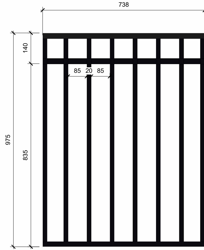
Railing type 1 Bay 1 - 737.5mm wide Bay 4 - Level 01 only - 775mm wide RAL9005
