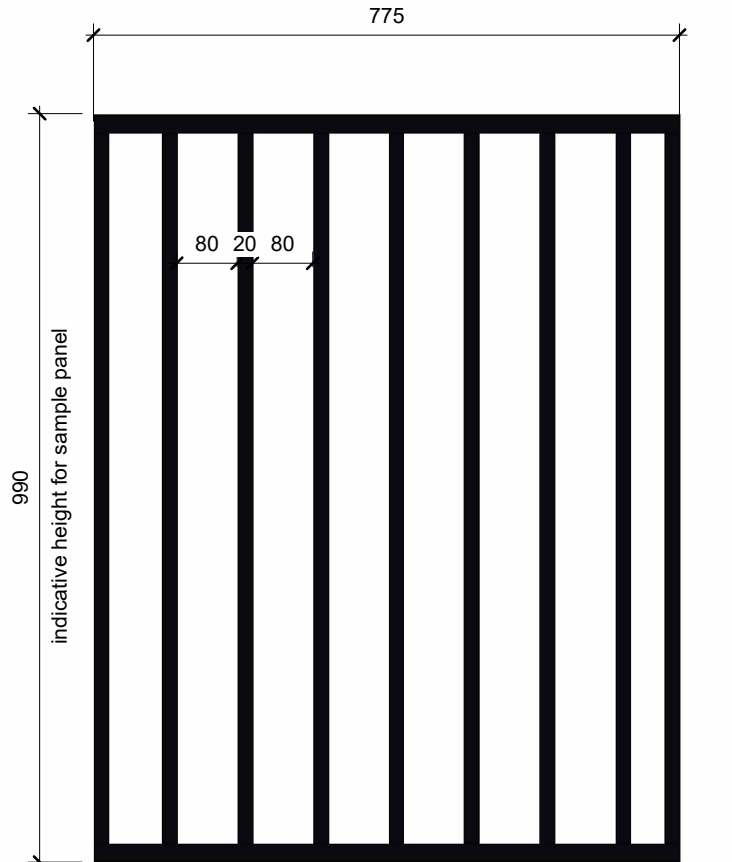
Railing type 3 Bay 4 - 900mm and 990mm high RAL9005
