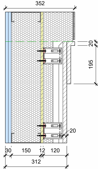
4 Typical Section 1 : 10
