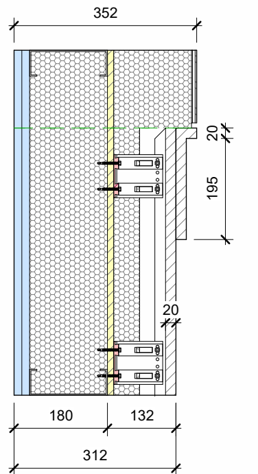
3 Typical Section 1 : 10
