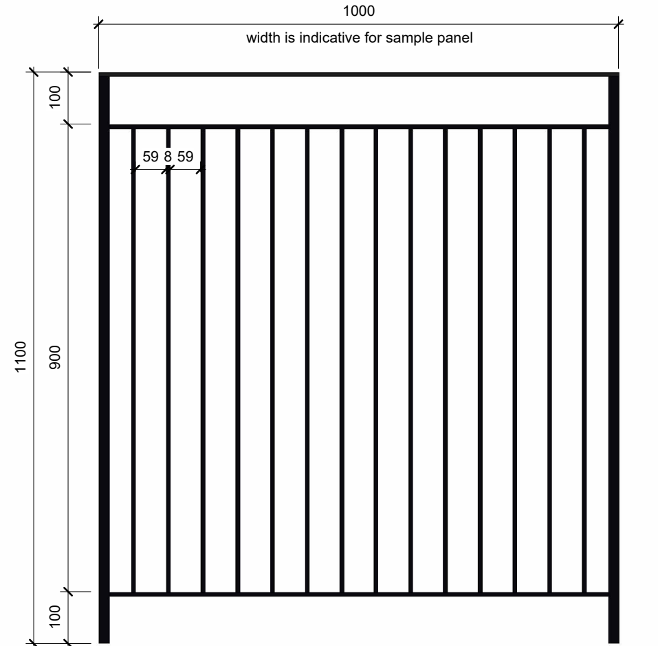
Railing type 5 Metal Railing on roof terraces RAL9005
