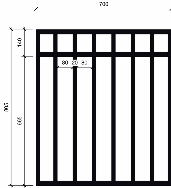
Railing type 2 Bay 3 - Level 01 only RAL9005
