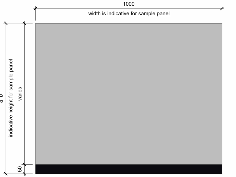
Railing type 7 Glass balustrade without handrail height of balustrade varies
