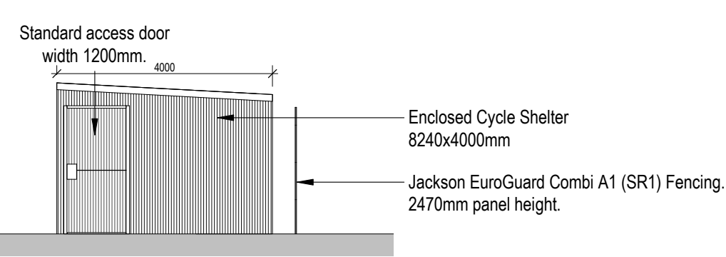
Cycle Shelter - Front Elevation
