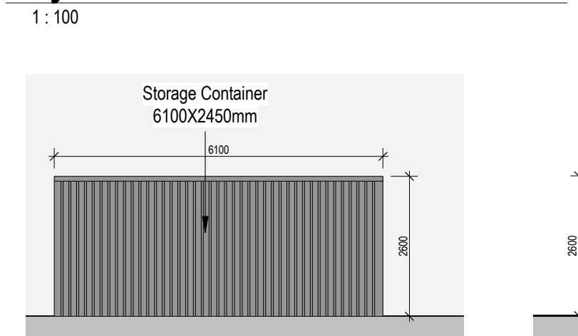
Container 01 - Front & Side Elevation
