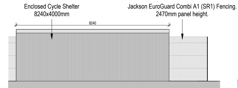
Cycle Shelter - Side Elevation
