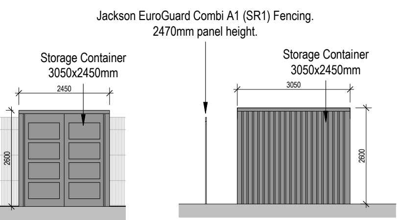
Container 02 - Front & Side Elevation
