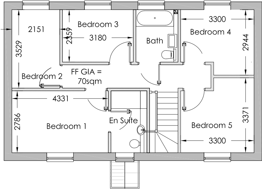
01 PROPOSED FIRST FLOOR PLAN 1:100
