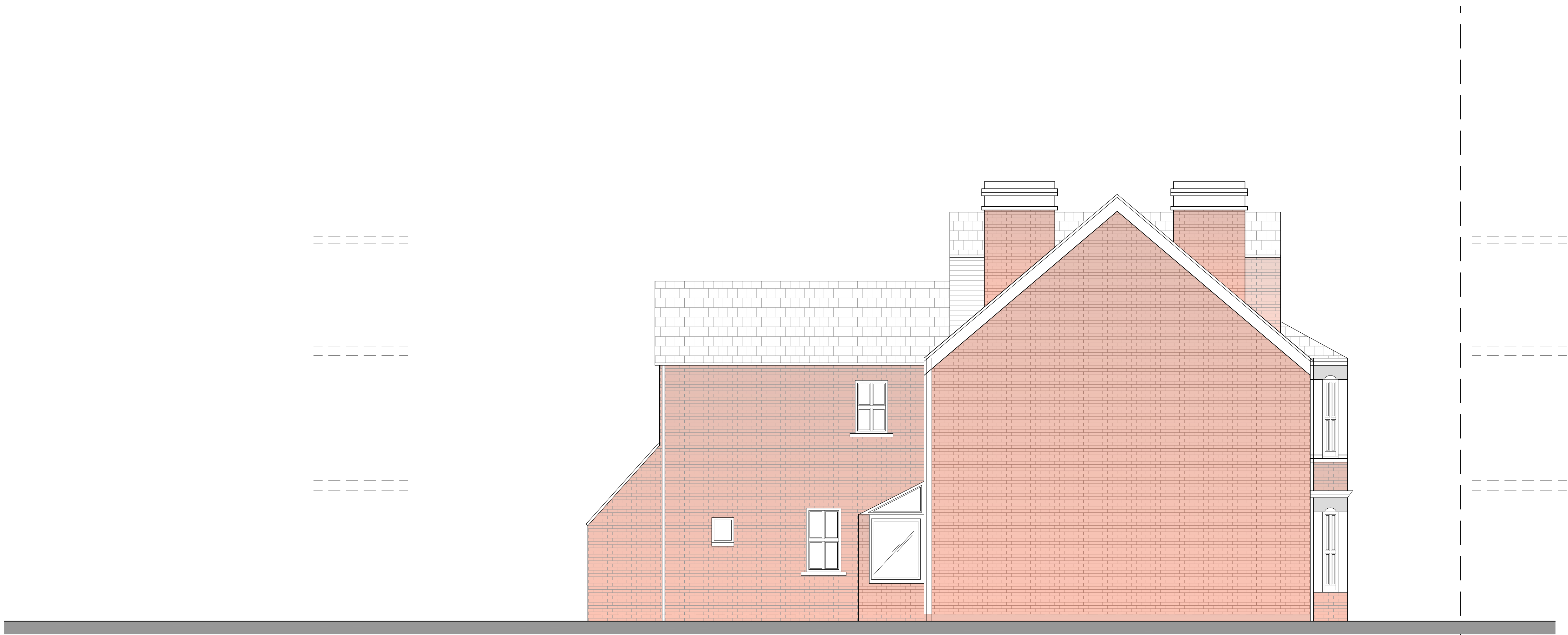
Existing Side Elevation Scale 1:50
