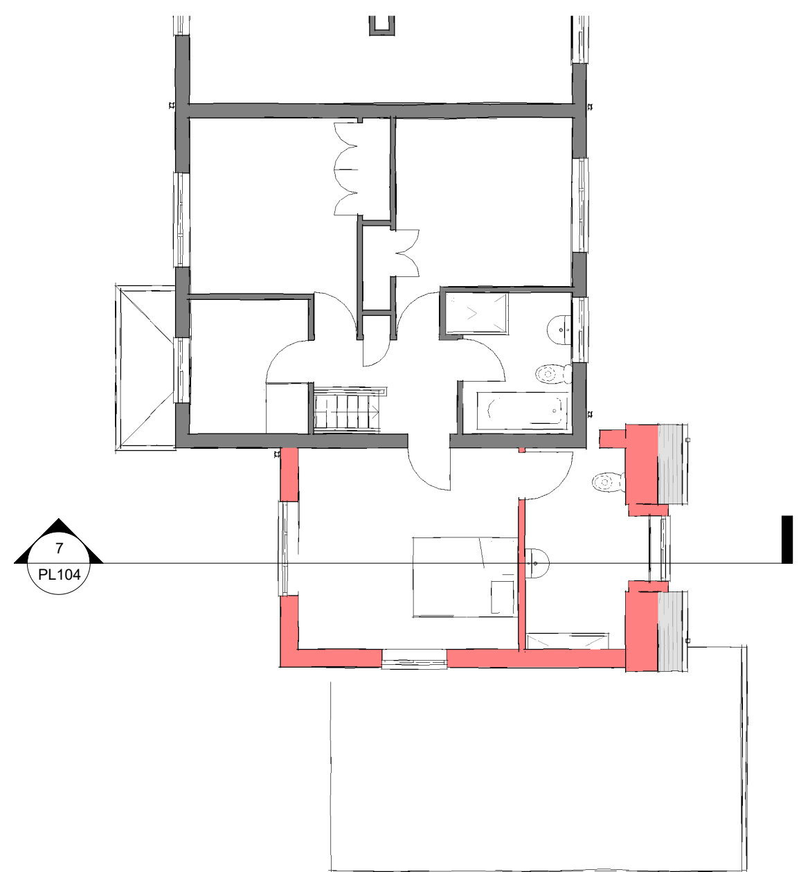
3 First Floor 1 : 100
