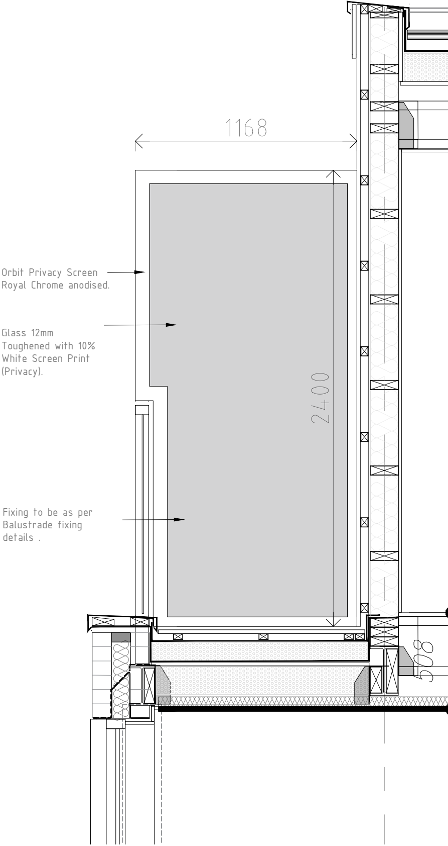
PRIVACY SCREEN DETAIL 1:20
